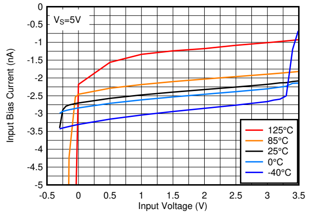
Figure 3-22. Input Bias Current vs. Input Voltage at 5\text{ V}
