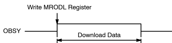
Figure 23. OTP Data Download Timing after an MRODL Command
