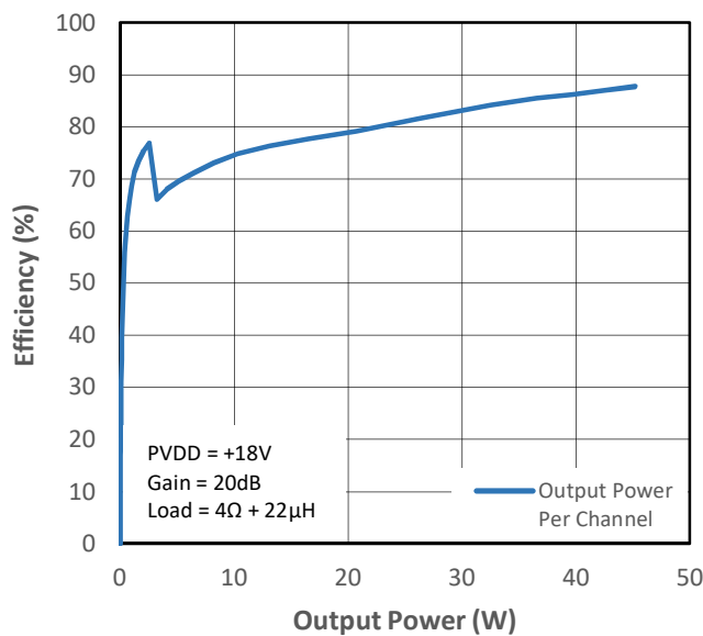
Figure 10-11 PMP2 Efficiency (VDD+PVDD) vs Output Power
