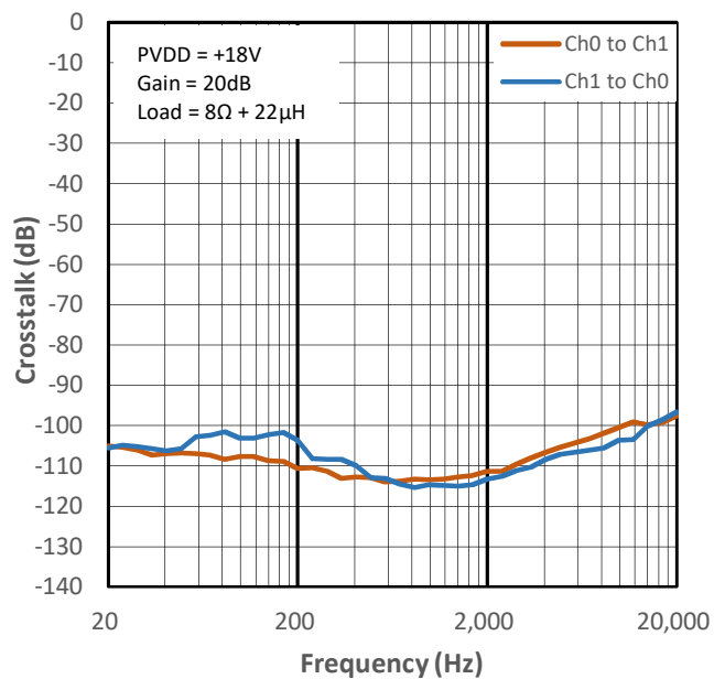
Figure 11-34 Crosstalk vs Frequency for PMP1
