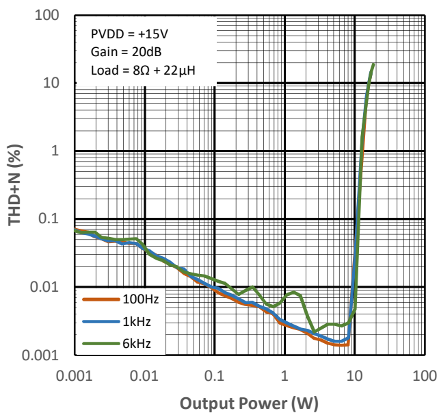
Figure 13-3 THD+N vs. Output Power for PMP2
