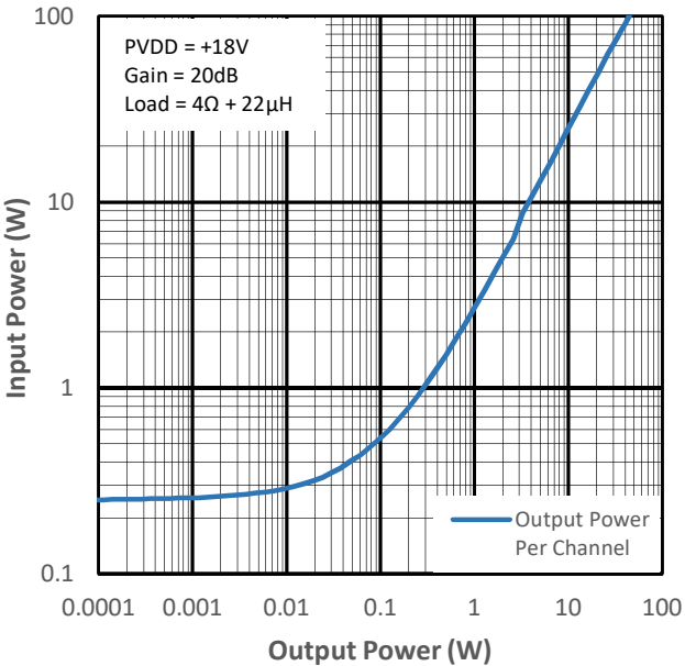
Figure 10-13 Input Power vs Output Power for PMP0
