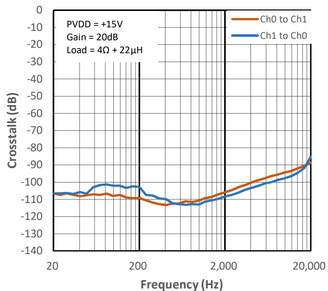
Figure 12-32 Crosstalk vs Frequency for PMP4
