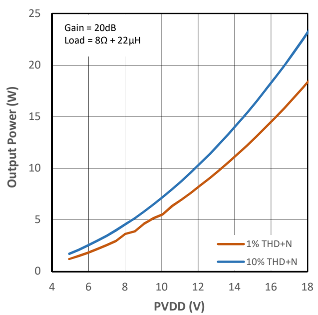
Figure 11-22 Output Power vs PVDD Voltage for PMP1
