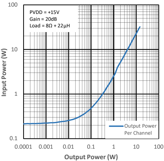
Figure 13-13 Input Power vs Output Power for PMP0
