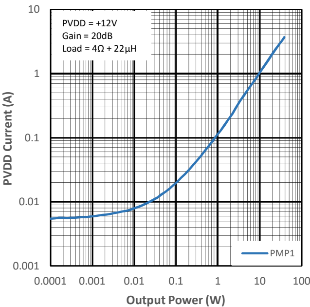
Figure 14-18 PVDD Current vs Output Power for PMP1
