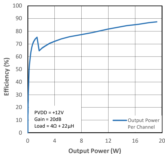
Figure 14-11 PMP2 Efficiency (VDD+PVDD) vs Output Power
