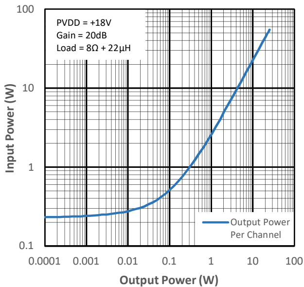
Figure 11-16 Input Power vs Output Power for PMP4
