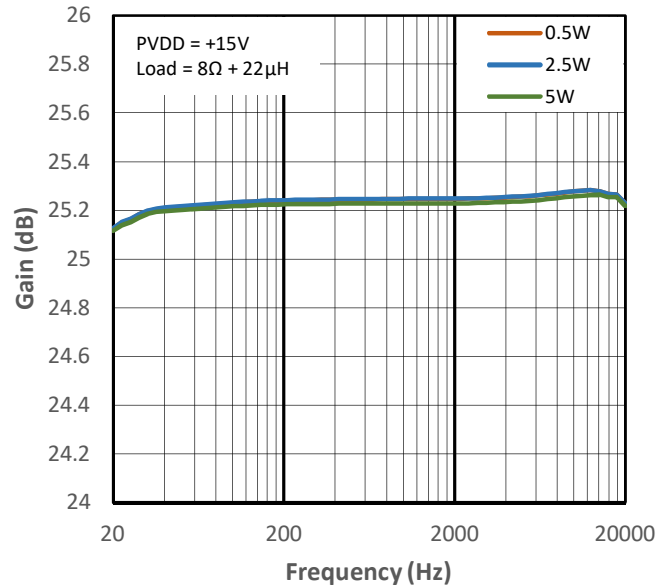
Figure 13-27 High Gain vs Frequency for PMP2
