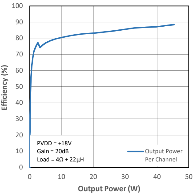
Figure 10-10 PMP1 Efficiency (VDD+PVDD) vs Output Power
