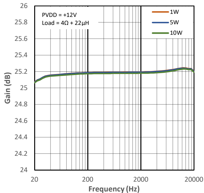
Figure 14-26 High Gain vs Frequency for PMP1
