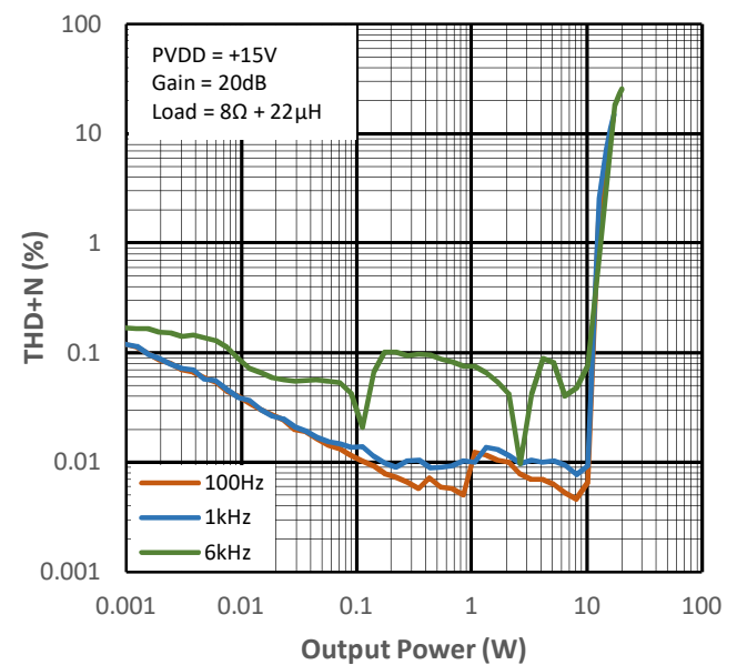
Figure 13-4 THD+N vs. Output Power for PMP4
