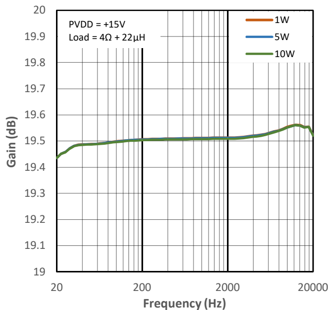
Figure 12-22 Low Gain vs Frequency for PMP1
