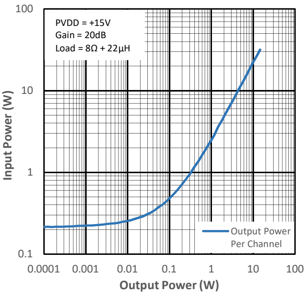
Figure 13-16 Input Power vs Output Power for PMP4
