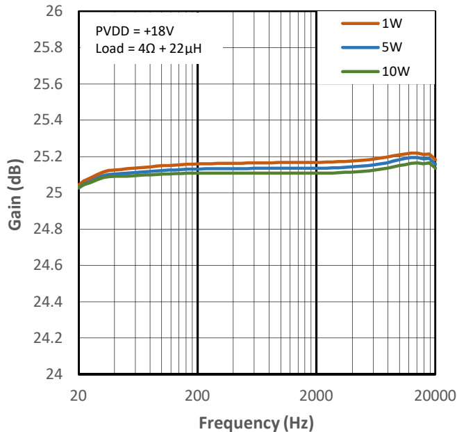
Figure 10-30 High Gain vs Frequency for PMP1
