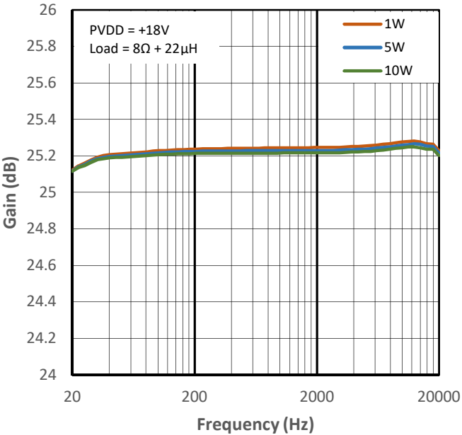
Figure 11-30 High Gain vs Frequency for PMP1
