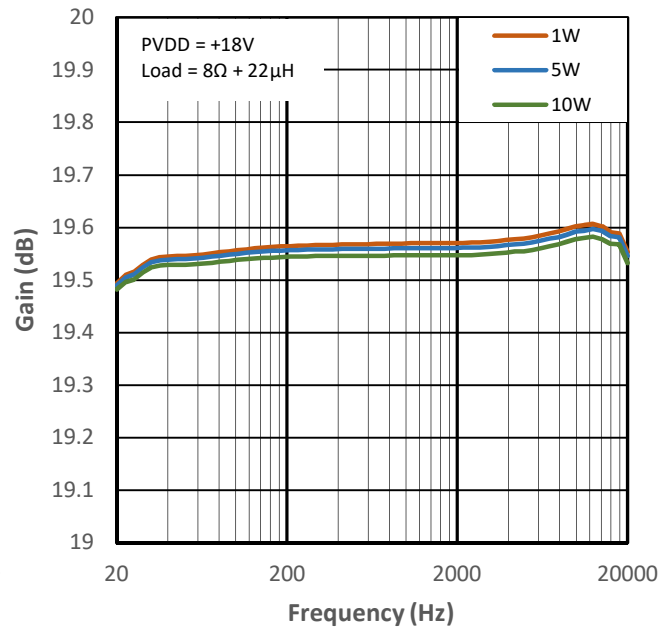
Figure 11-26 Low Gain vs Frequency for PMP1
