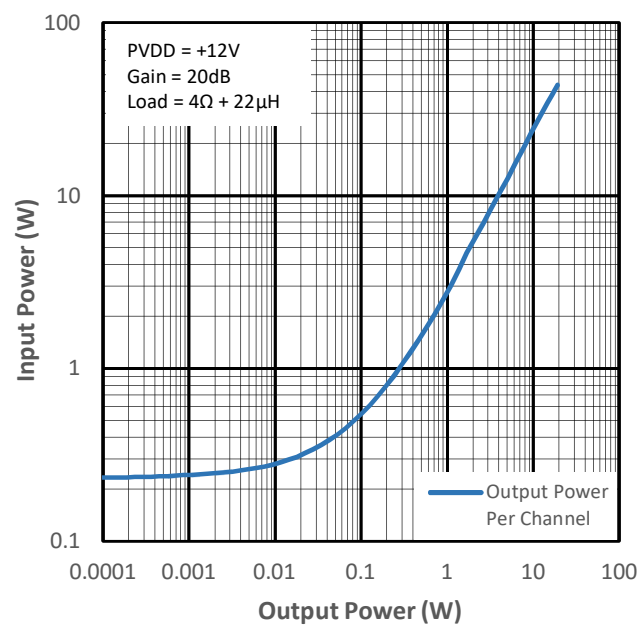
Figure 14-14 Input Power vs Output Power for PMP1
