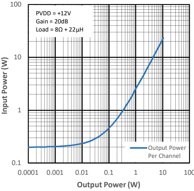
Figure 15-16 Input Power vs Output Power for PMP4
