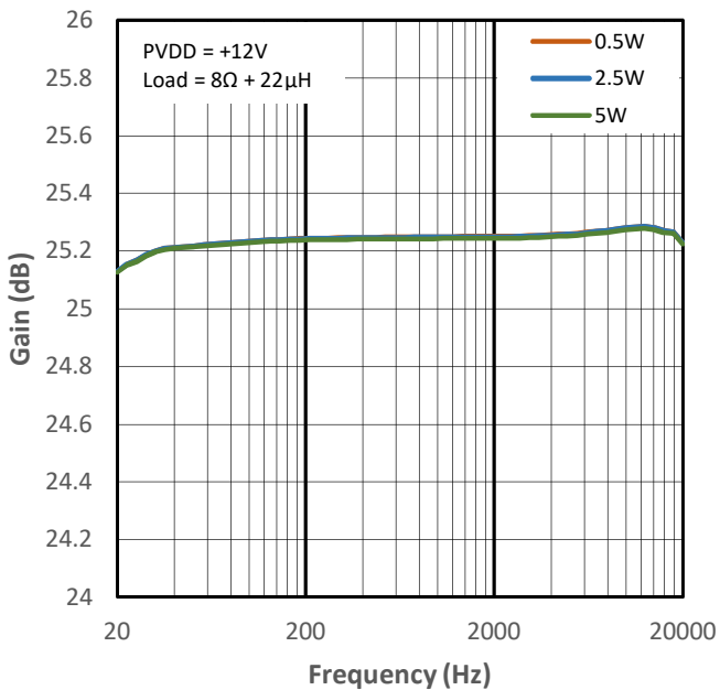
Figure 15-26 High Gain vs Frequency for PMP1
