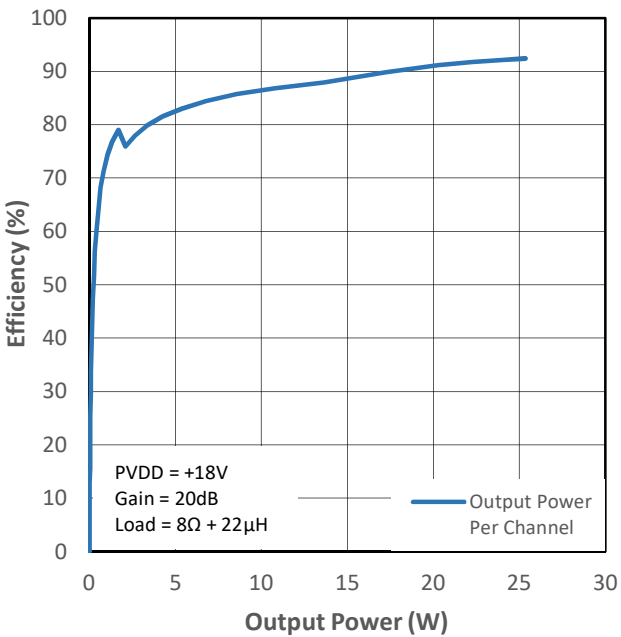
Figure 11-10 PMP1 Efficiency (VDD+PVDD) vs Output Power
