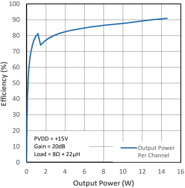
Figure 13-9 PMP0 Efficiency (VDD+PVDD) vs Output Power
