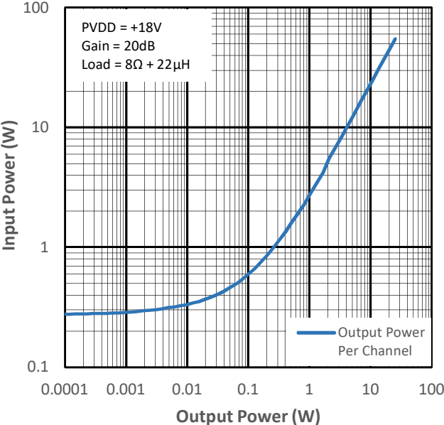
Figure 11-14 Input Power vs Output Power for PMP1
