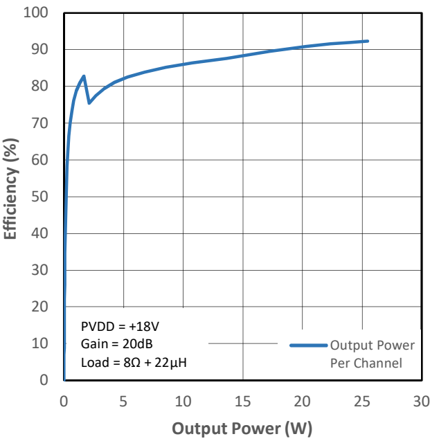
Figure 11-9 PMP0 Efficiency (VDD+PVDD) vs Output Power
