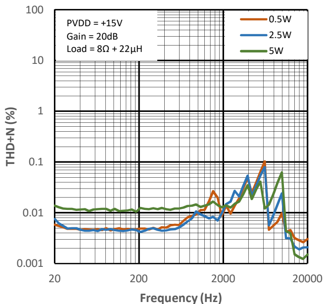
Figure 13-5 THD+N vs Frequency for PMP0
