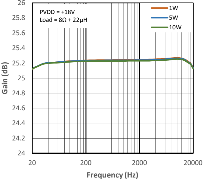
Figure 11-32 High Gain vs Frequency for PMP4
