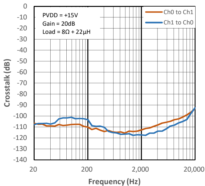
Figure 13-36 Crosstalk vs Frequency for PMP4
