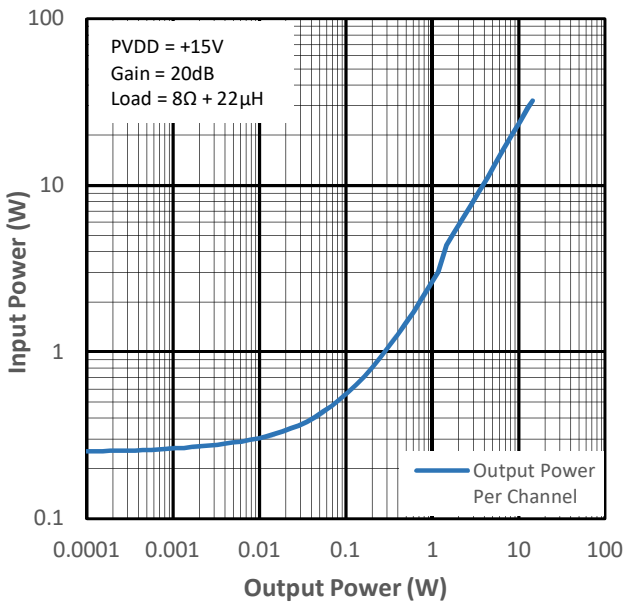
Figure 13-15 Input Power vs Output Power for PMP2
