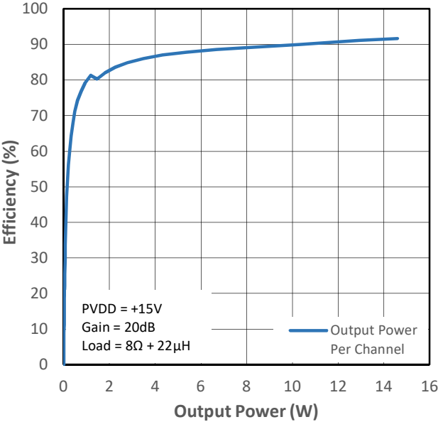
Figure 13-12 PMP4 Efficiency (VDD+PVDD) vs Output Power
