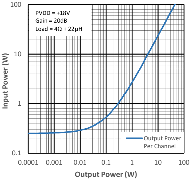
Figure 10-16 Input Power vs Output Power for PMP4
