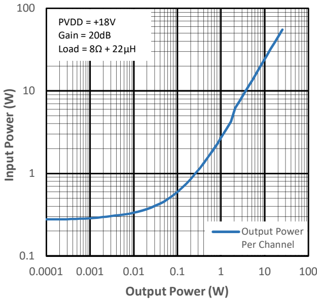
Figure 11-15 Input Power vs Output Power for PMP2
