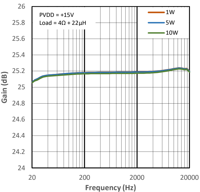
Figure 12-26 High Gain vs Frequency for PMP1
