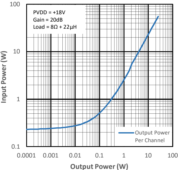
Figure 11-13 Input Power vs Output Power for PMP0
