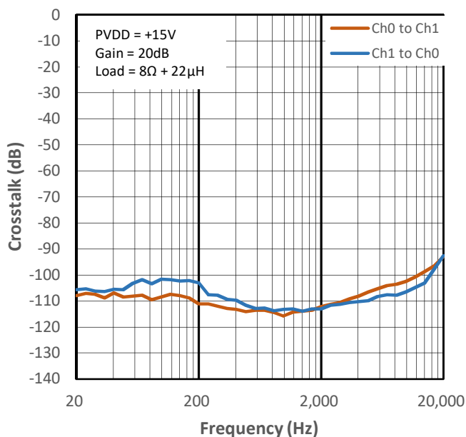
Figure 13-29 Crosstalk vs Frequency for PMP0
