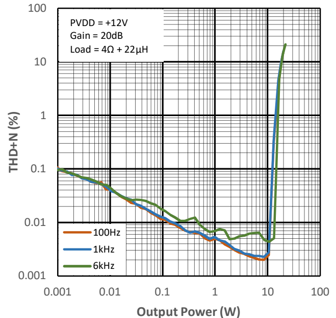
Figure 14-2 THD+N vs. Output Power for PMP1
