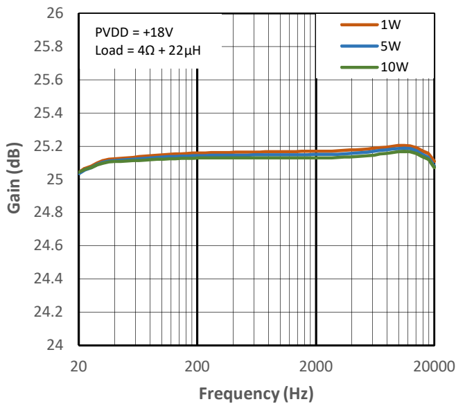
Figure 10-32 High Gain vs Frequency for PMP4
