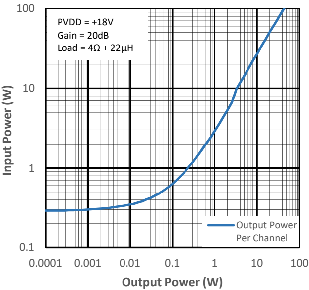
Figure 10-15 Input Power vs Output Power for PMP2
