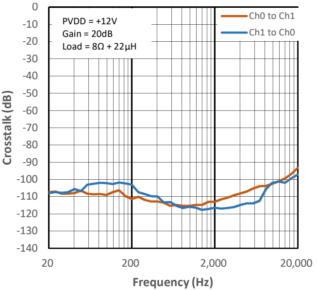
Figure 15-36 Crosstalk vs Frequency for PMP4
