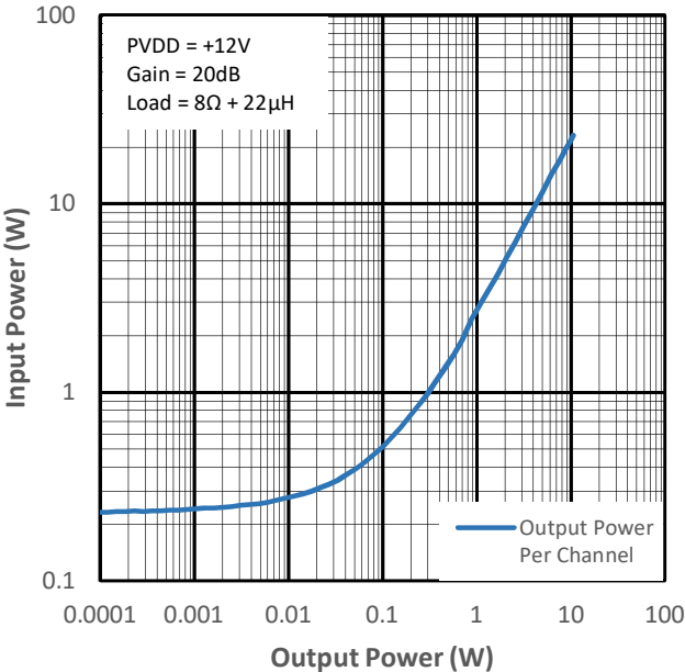
Figure 15-14 Input Power vs Output Power for PMP1
