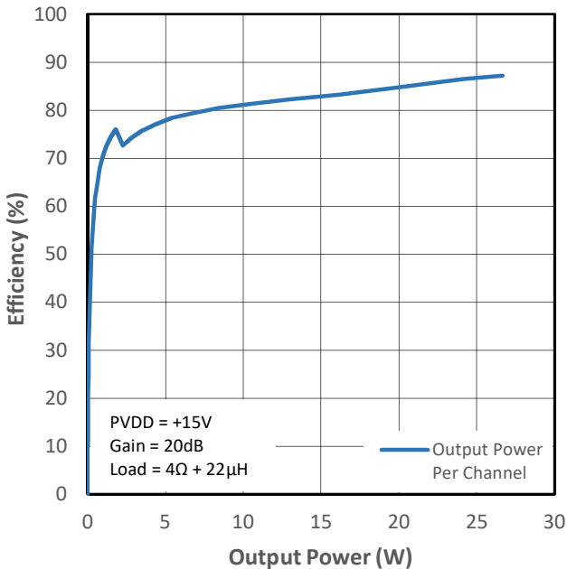
Figure 12-10 PMP1 Efficiency (VDD+PVDD) vs Output Power
