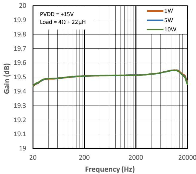
Figure 12-24 Low Gain vs Frequency for PMP4
