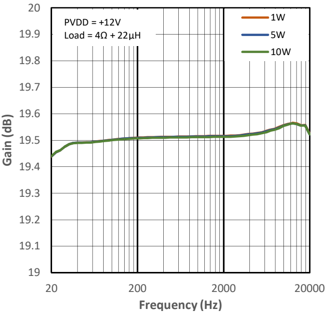
Figure 14-22 Low Gain vs Frequency for PMP1
