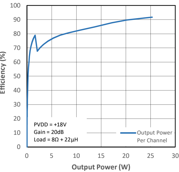
Figure 11-11 PMP2 Efficiency (VDD+PVDD) vs Output Power
