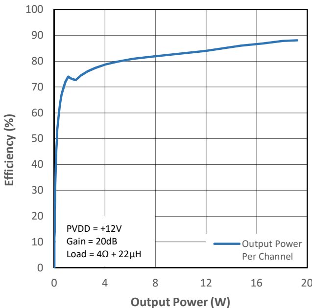
Figure 14-10 PMP1 Efficiency (VDD+PVDD) vs Output Power
