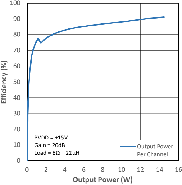
Figure 13-10 PMP1 Efficiency (VDD+PVDD) vs Output Power
