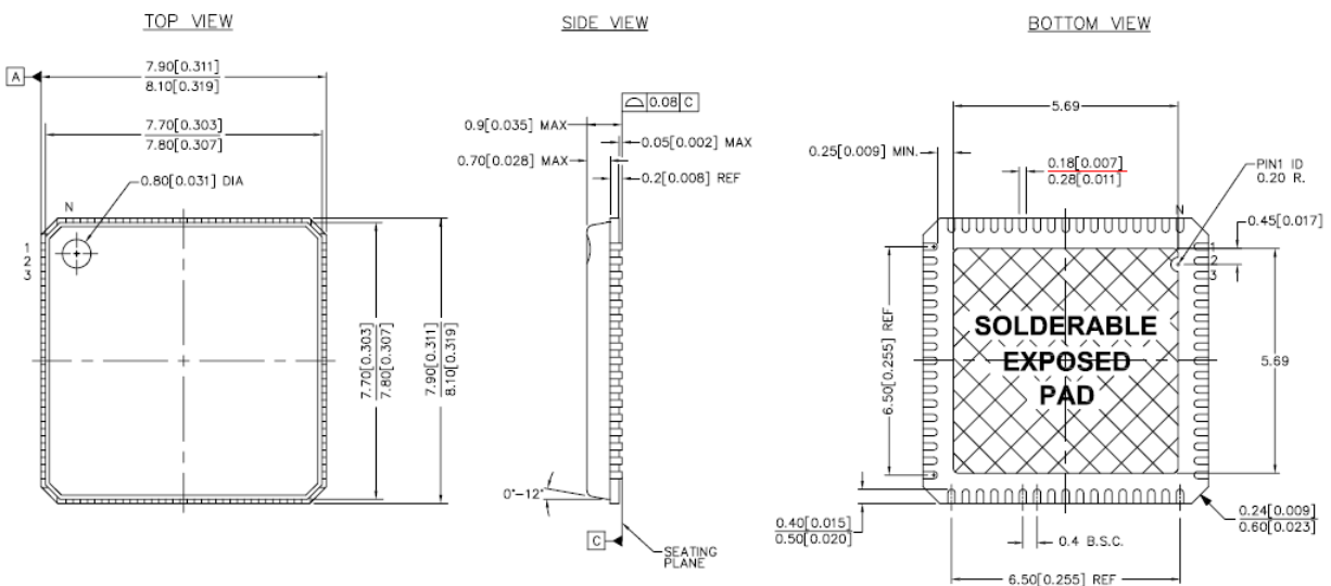
Figure 10-3. 68-Pin (8x8 mm x 0.89 mm) QFN
