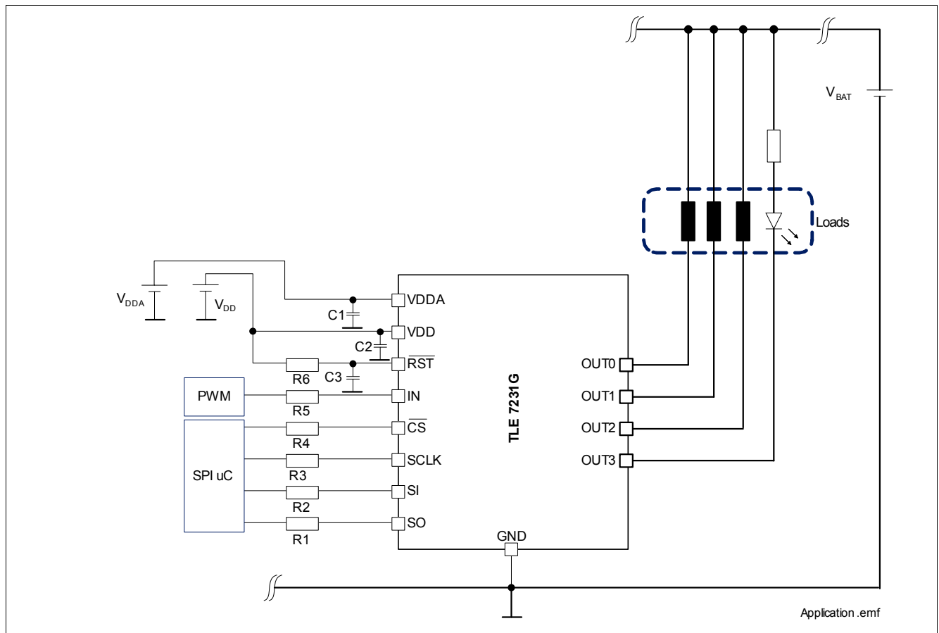
Figure 14 Application Diagram
