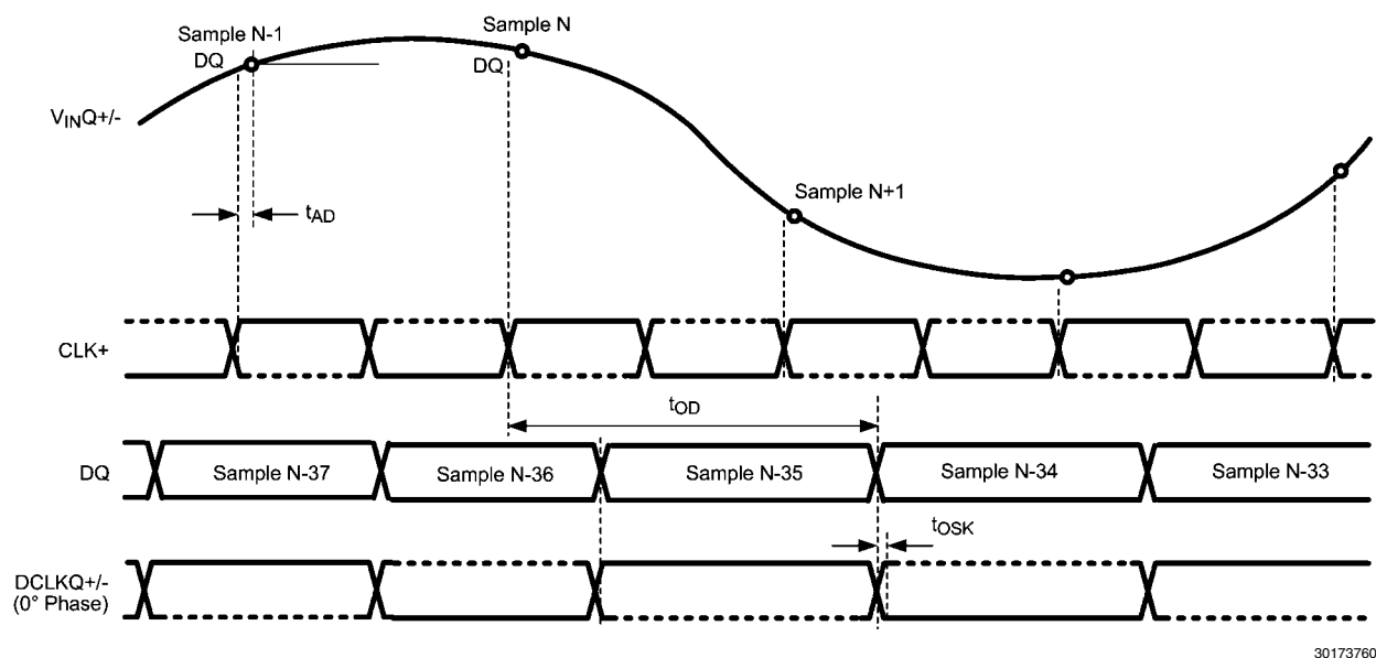
FIGURE 5. Clocking in Non-Demux Non-DES Mode*
