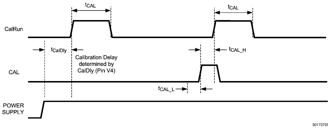
FIGURE 9. Power-on and On-Command Calibration Timing
