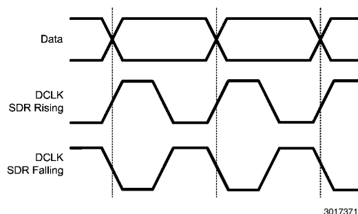
FIGURE 14. SDR DCLK-to-Data Phase Relationship
