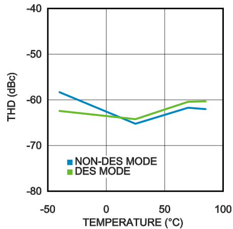
THD vs. TEMPERATURE (ADC12D2000RF)
