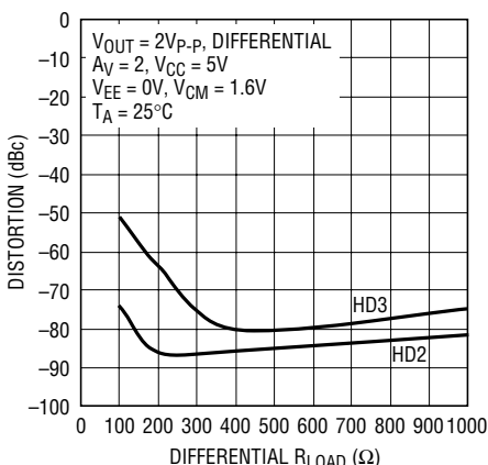
Harmonic Distortion vs Load, 30MHz, Differential Input
