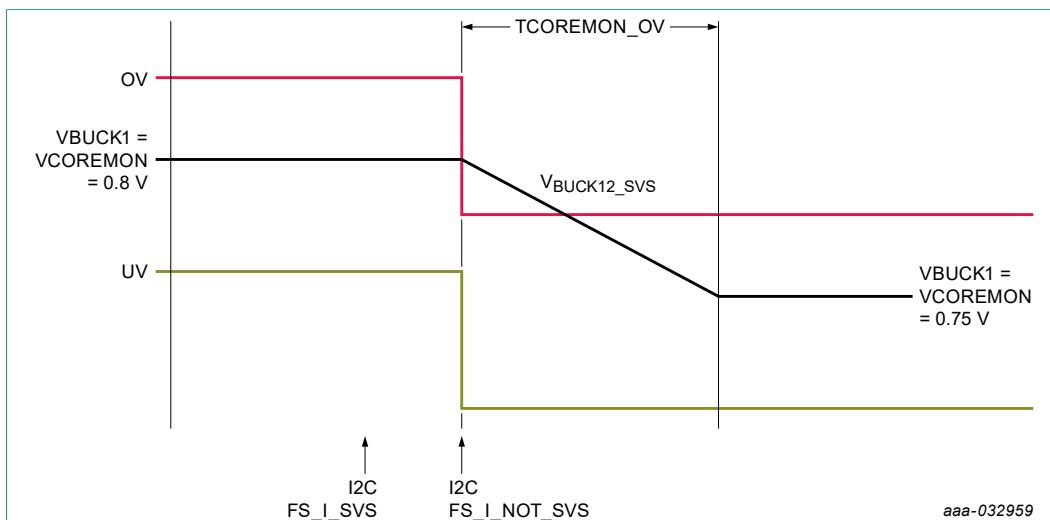
Figure 41. SVS principle
