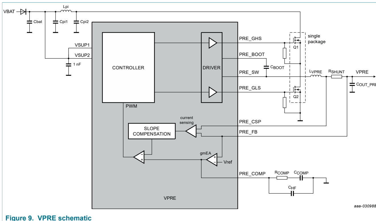
Figure 9. VPRE schematic
