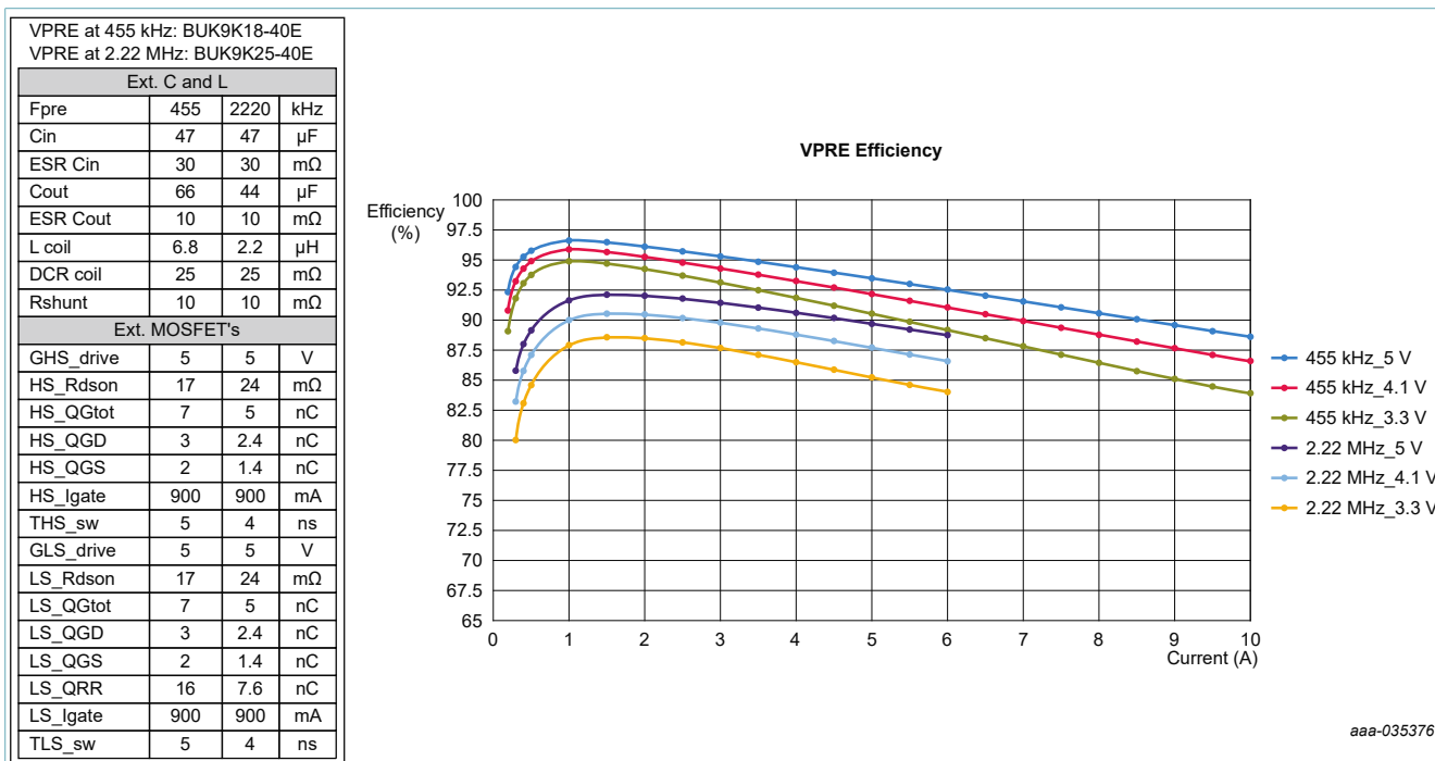
Figure 14. VPRE theoretical efficiency
