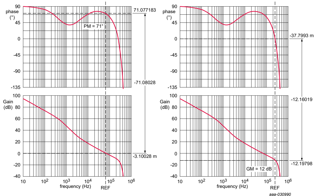
Figure 11. Phase and gain margin simulation
