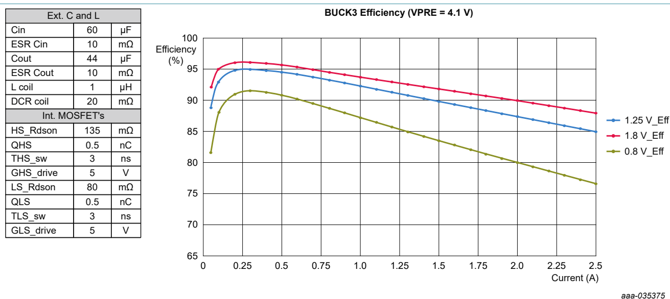
Figure 26. BUCK3 theoretical efficiency
