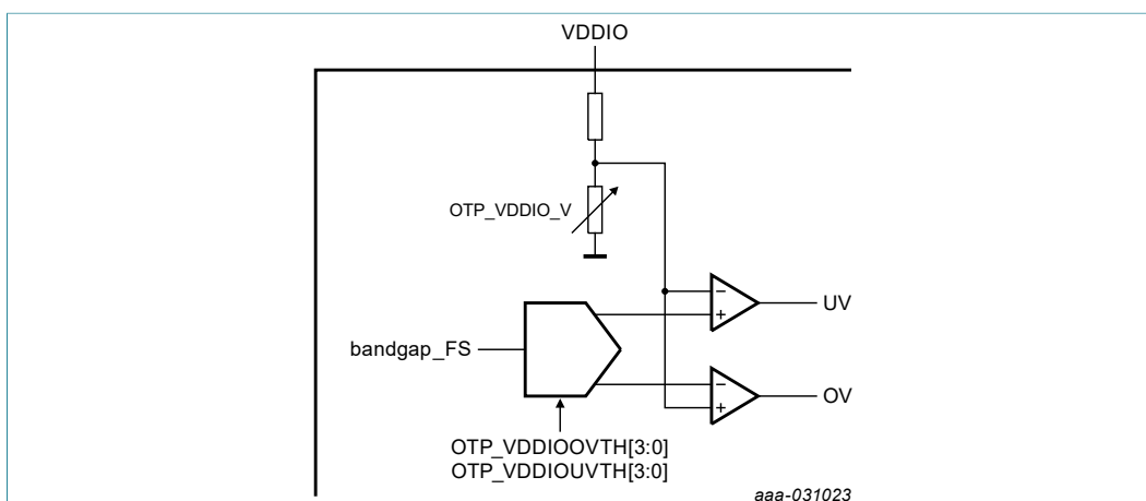
Figure 42. VDDIO monitoring principle
