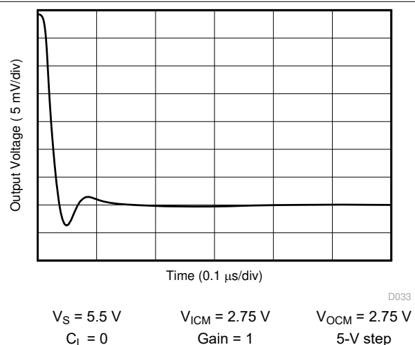
Figure 7-34. Large Signal Settling Time (Negative)
