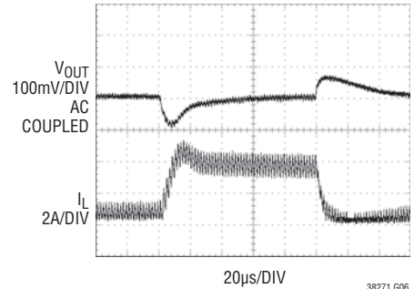
FIGURE 13 CIRCUIT V_{OUT} = 3.3V
