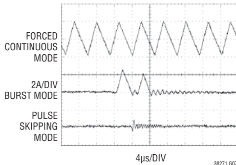
FIGURE 13 CIRCUIT V_{OUT} = 3.3V I_{LOAD} = 300\mu A
