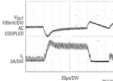
FIGURE 13 CIRCUIT V_{OUT} = 3.3V
