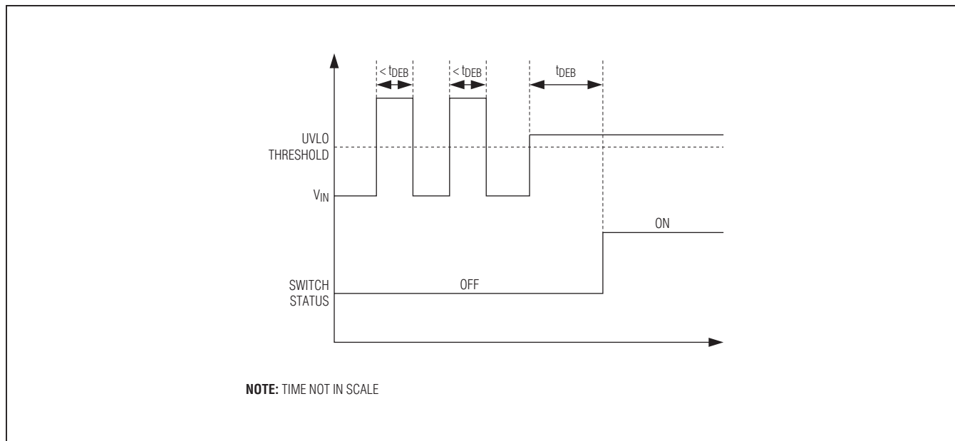
Figure 4. Debounce Timing
