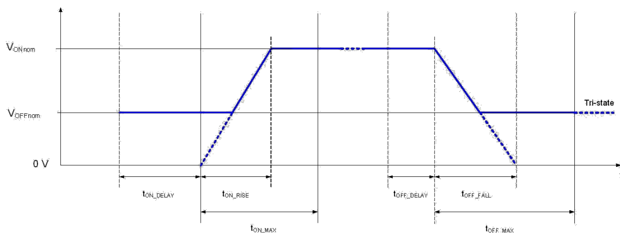
Figure 9: Power Sequencing With Non-Zero Off Voltage
