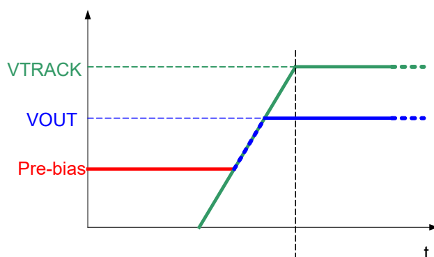
Figure 10: Power Sequencing Using VTRACK With Bias Voltage On VOUT
