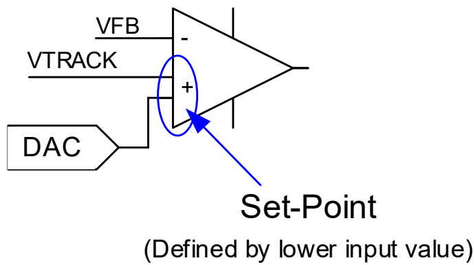
Figure 11: VTRACK Circuitry
