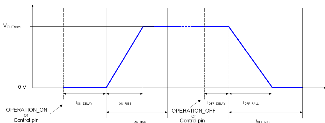
Figure 8: Power Sequencing
