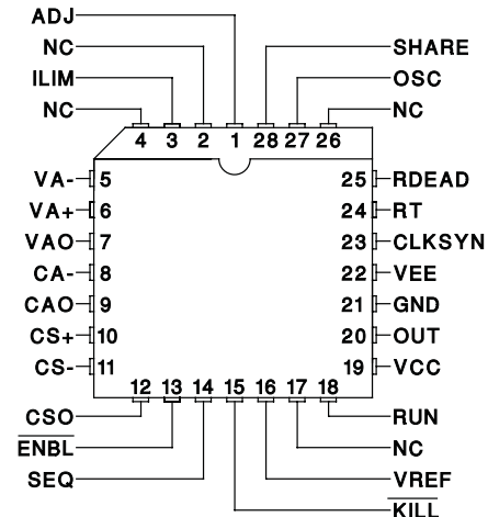
PLCC-28 (Top View) Q Package
