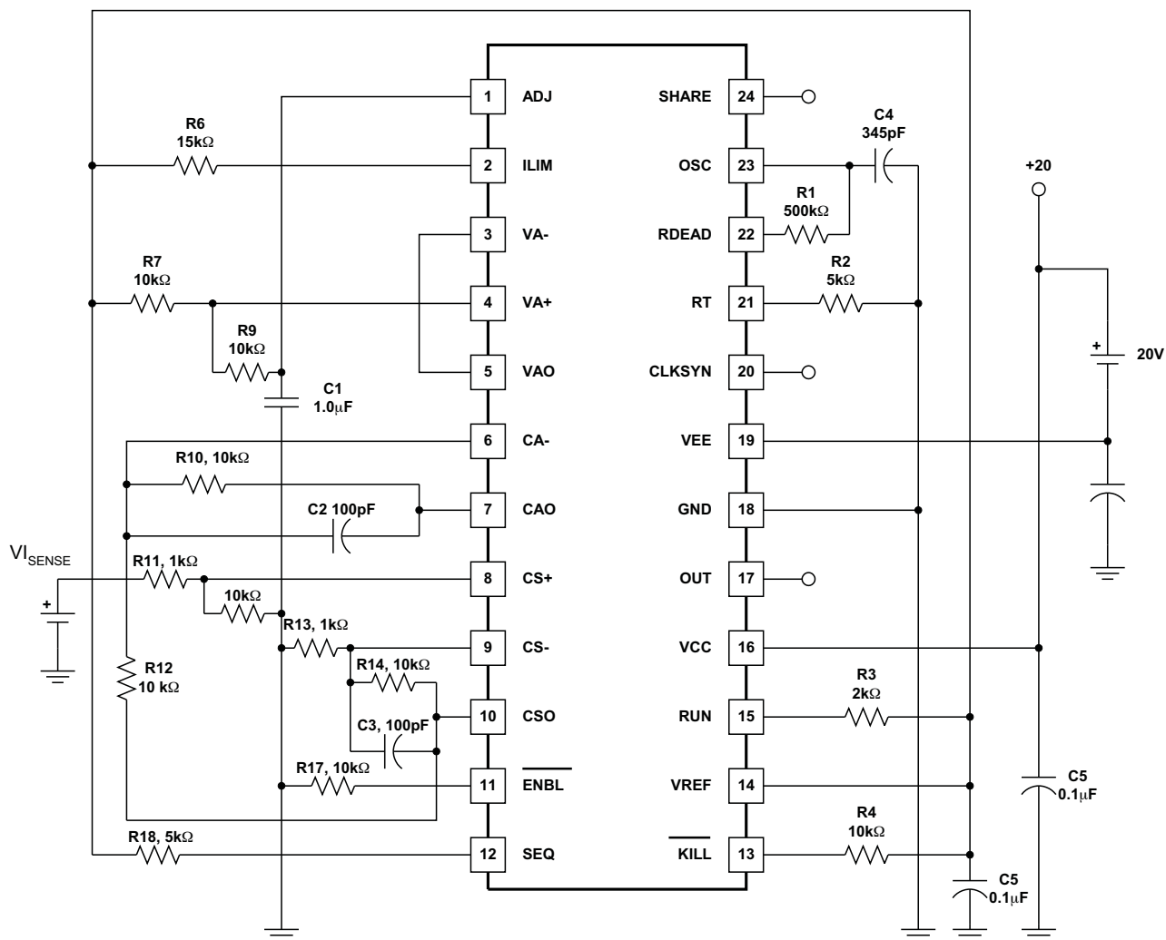
Figure 9. Open Loop Circuit
