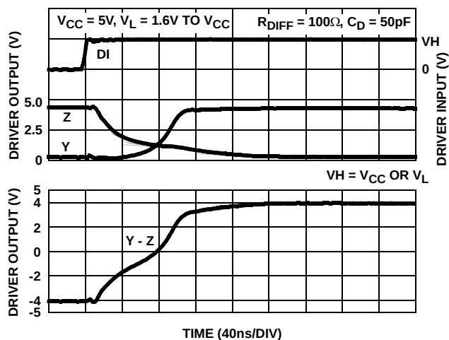
FIGURE 21. DRIVER WAVEFORMS, LOW TO HIGH (ISL32372E, ISL32374E, ISL32179E)
