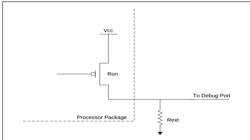
Figure 6. ITPCLKOUT[1:0] Output Buffer Diagram
