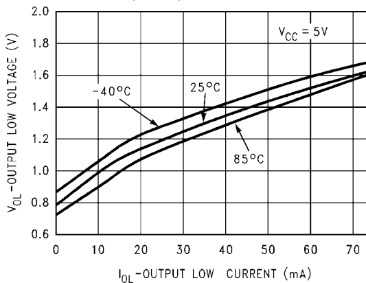
Driver V_{OL} vs I_{OL} vs Temperature
