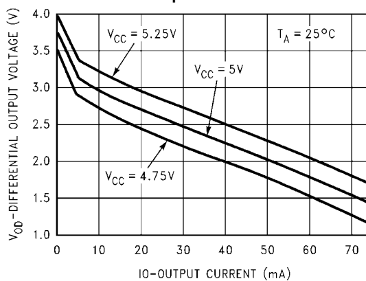
Differential Output Voltage vs Output Current
