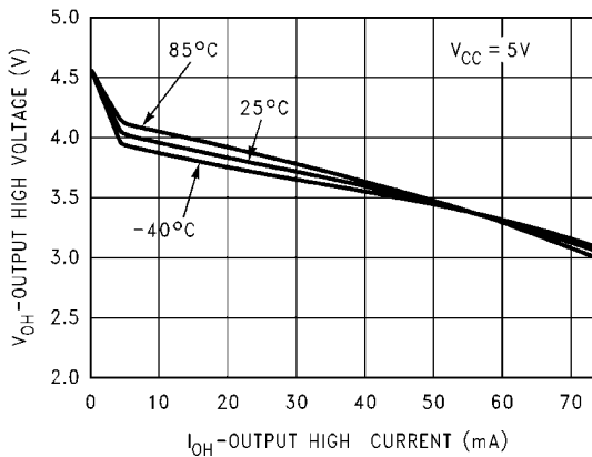
Driver V_{OH} vs I_{OH} vs Temperature
