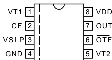
8-Pin SOIC (M)
