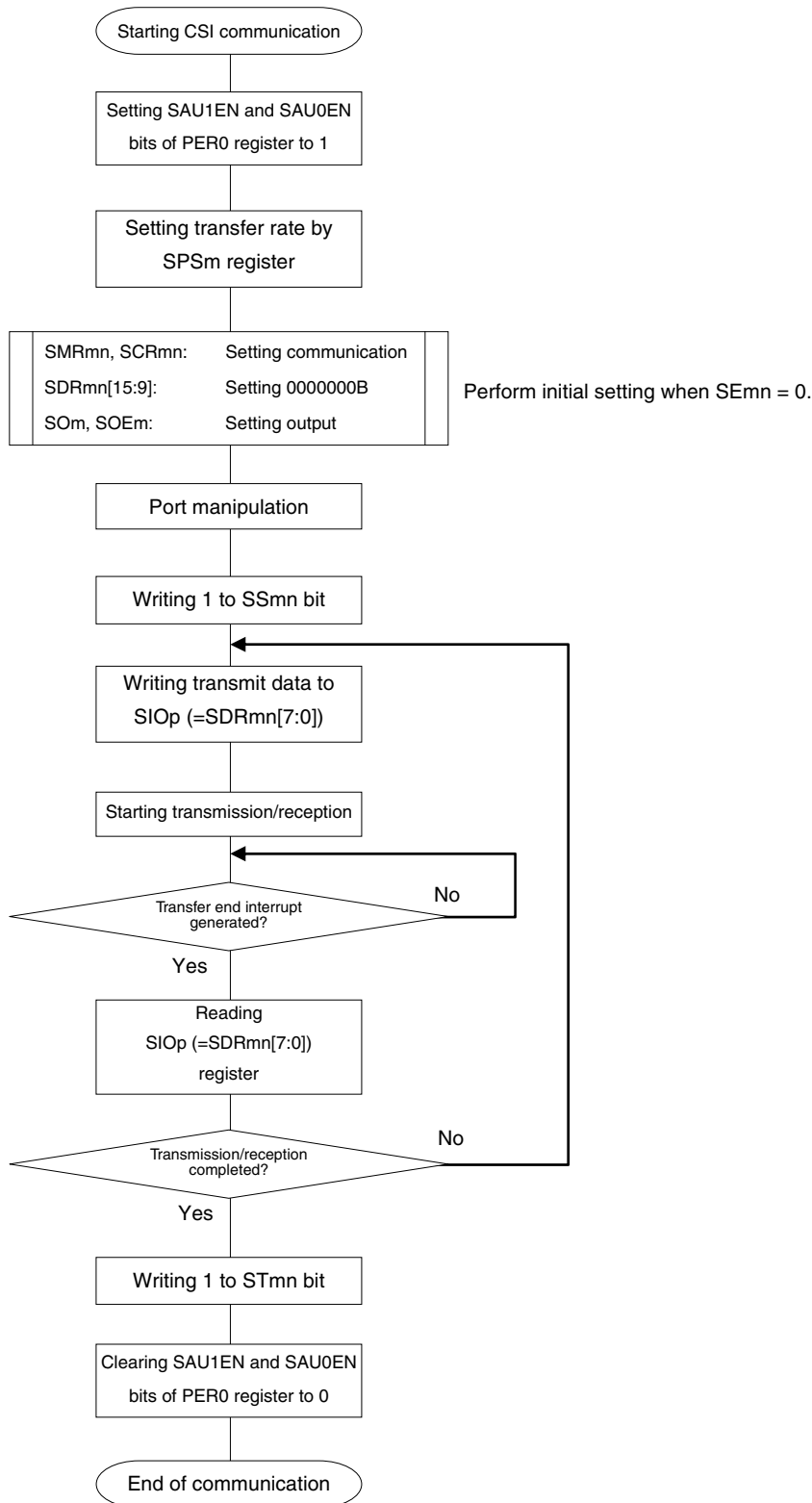
Figure 12-67. Flowchart of Slave Transmission/Reception (in Single-Transmission/Reception Mode)
