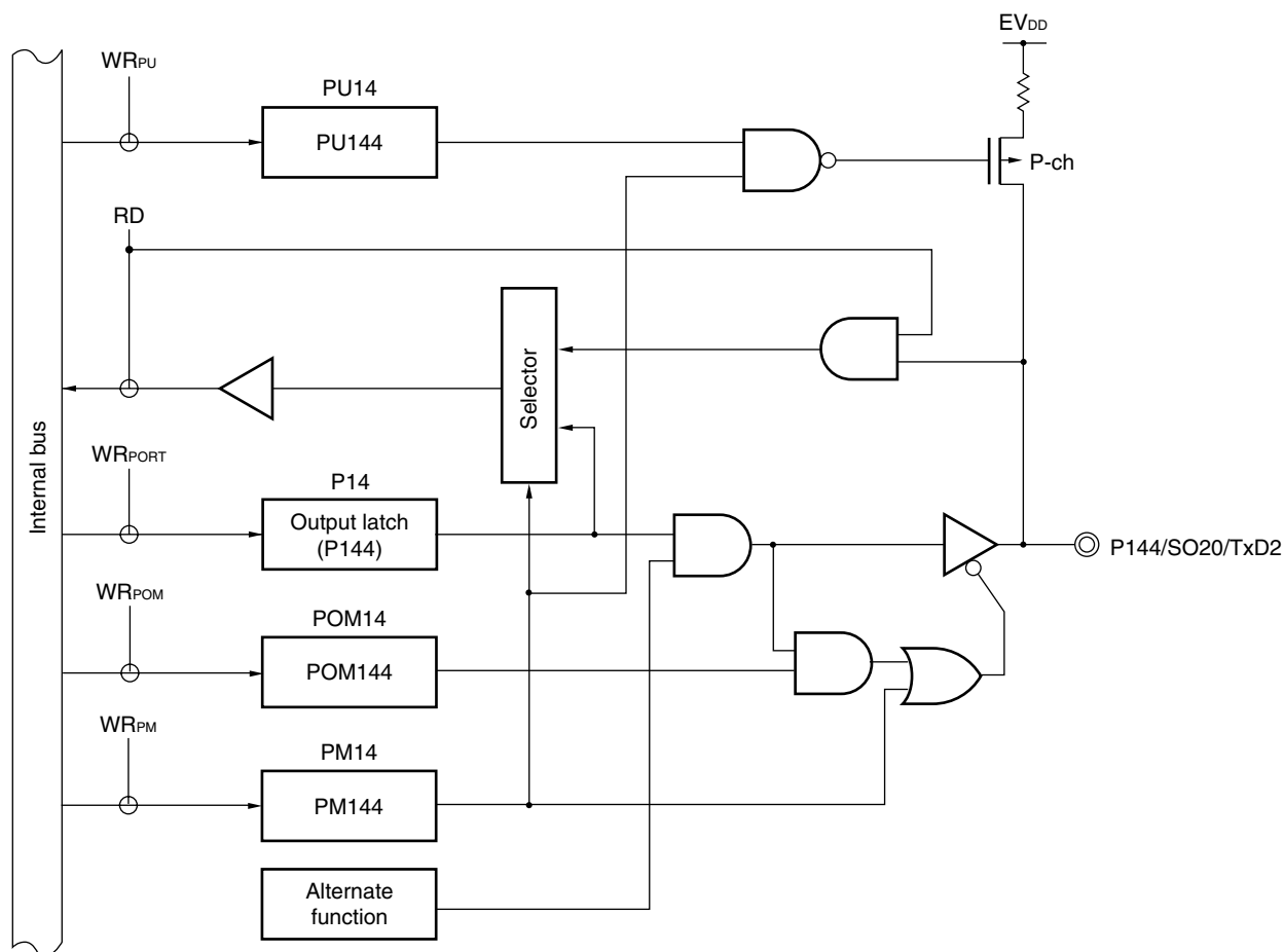
Figure 4-35. Block Diagram of P144
