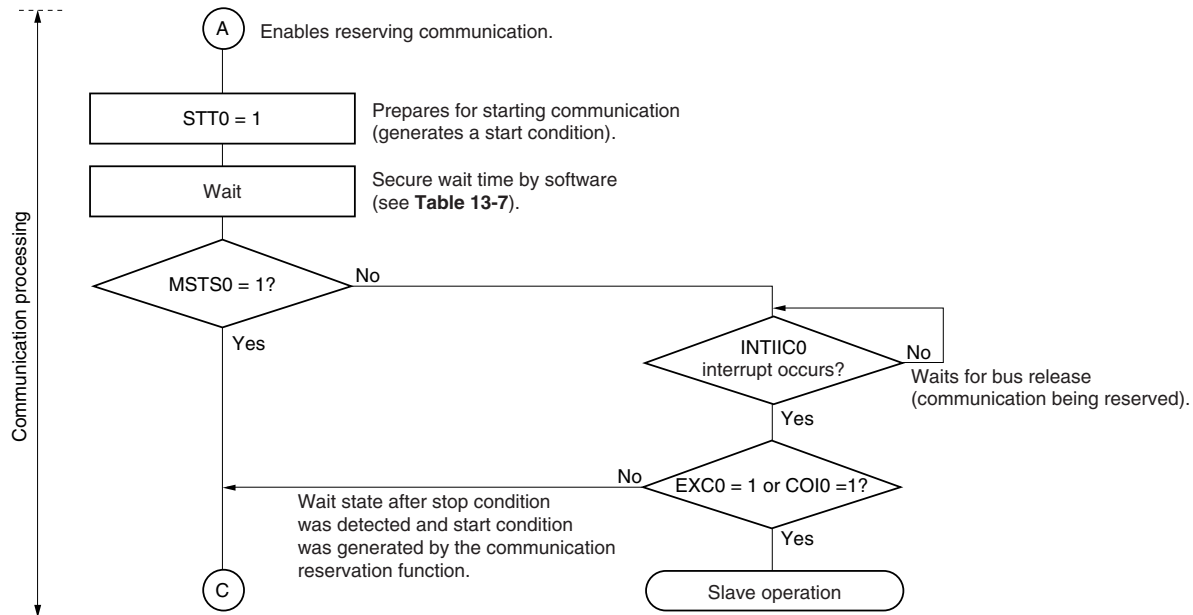
Figure 13-25. Master Operation in Multi-Master System (2/3)
