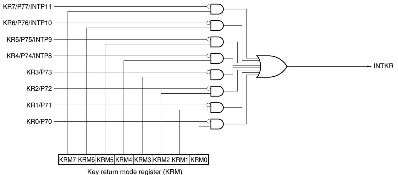
Figure 17-1. Block Diagram of Key Interrupt
