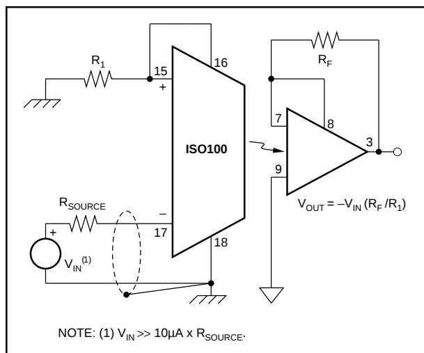
FIGURE 11. Bipolar Inverting.
