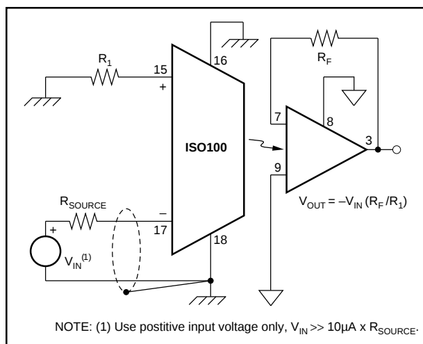
FIGURE 10. Unipolar Inverting.
