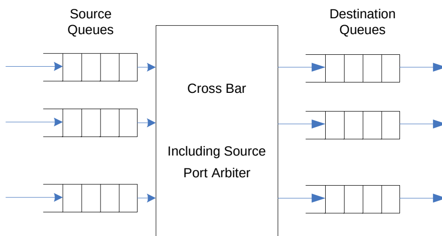
Figure 8-11. On-Chip Queuing
