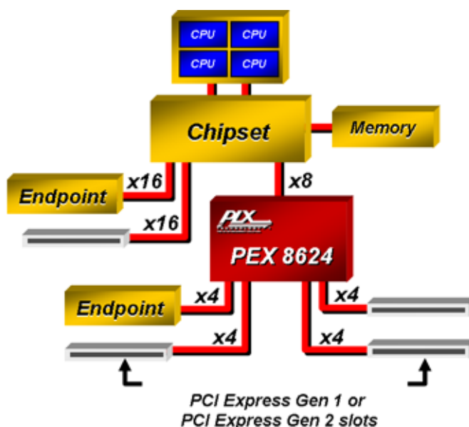
Figure 2-3. Fan-In/Fan-Out Usage
