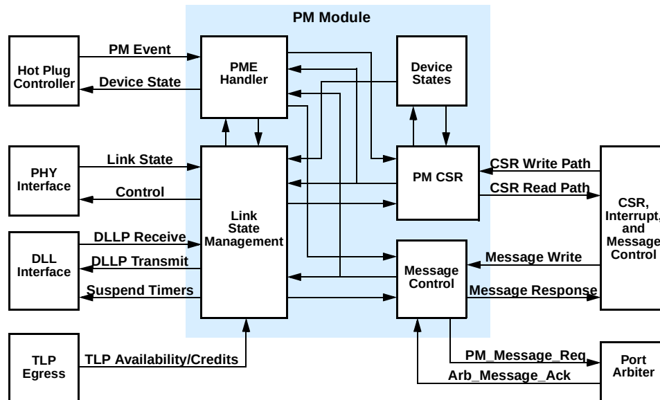
Figure 11-1. PM Module Functional Block Diagram
