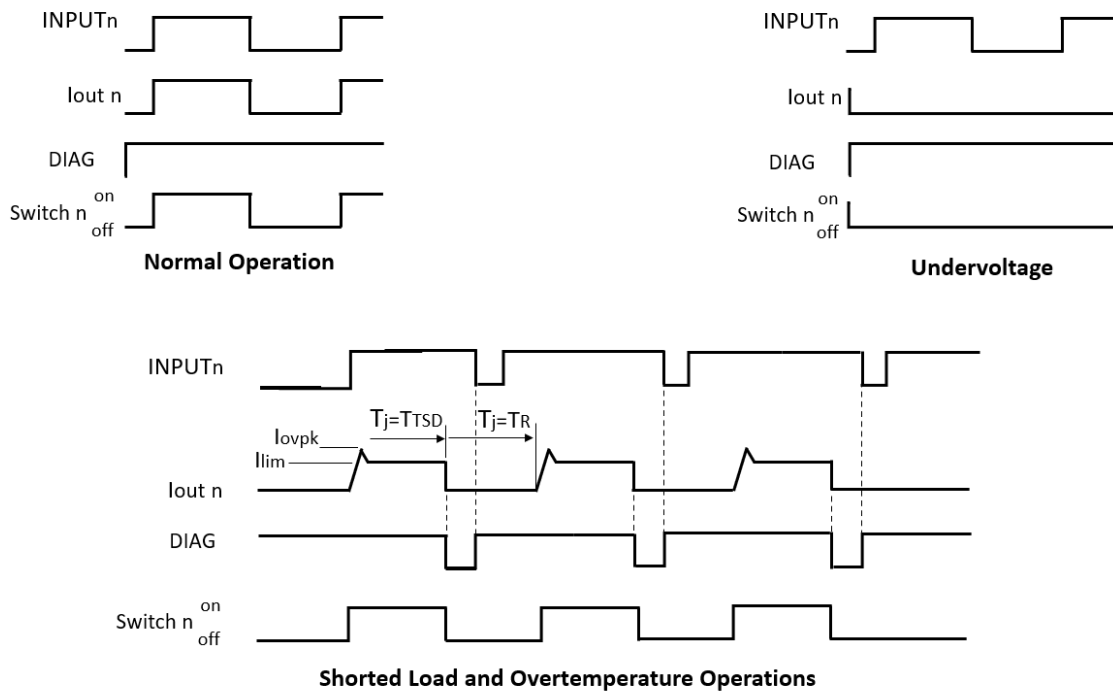
Figure 6. Switching waveforms
