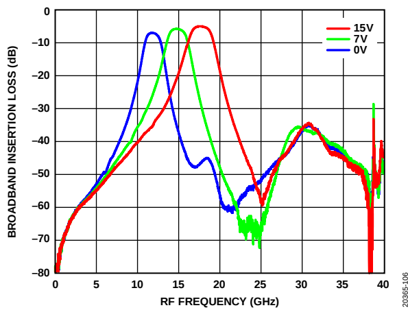
Figure 8. Broadband Insertion Loss vs. RF Frequency at Various Voltages
