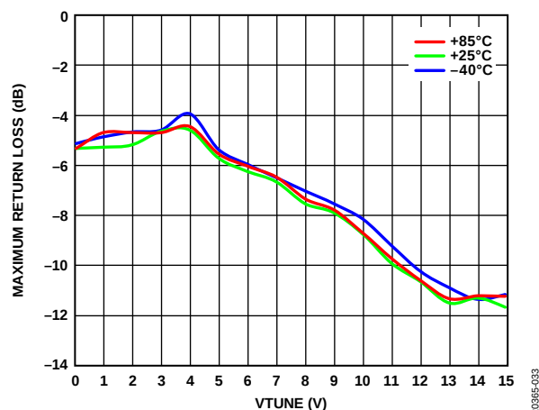
Figure 35. Maximum Return Loss in a 2 dB Bandwidth vs. VTUNE at Various Temperatures
