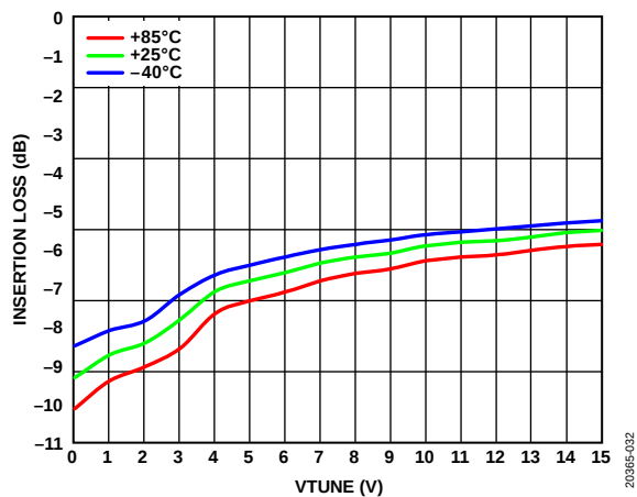
Figure 34. Insertion Loss vs. VTUNE at Various Temperatures
