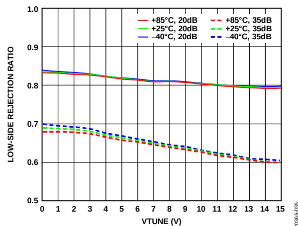
Figure 37. Low-Side Rejection vs. VTUNE at Various Temperatures and 20 dB and 35 dB
