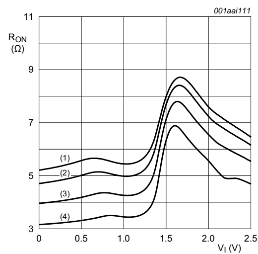
Fig 11. ON resistance as a function of input voltage; V_{CC} = 2.5 V; I_{SW} = 64 mA
