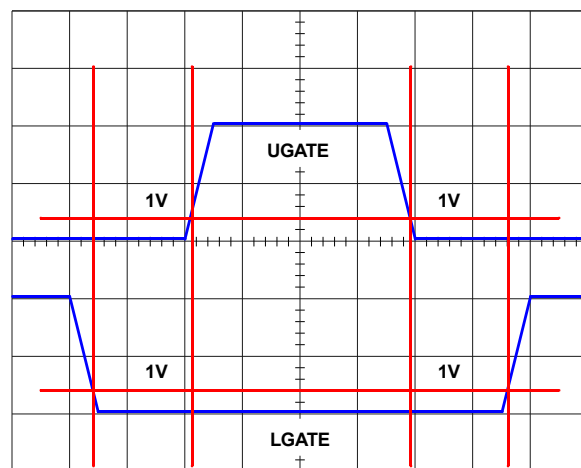
FIGURE 6. GATE DRIVER ADAPTIVE SHOOT-THROUGH
