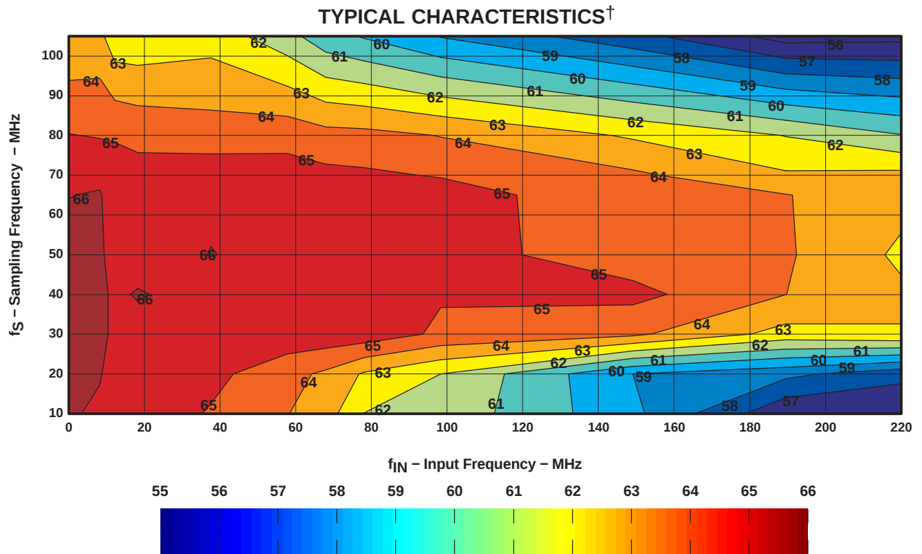
Figure 13. SNR– dBFS
