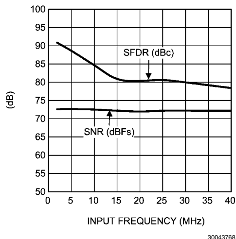
FIGURE 11. LMH6553/ADC14C105 SFDR and SNR Performance vs. Frequency
