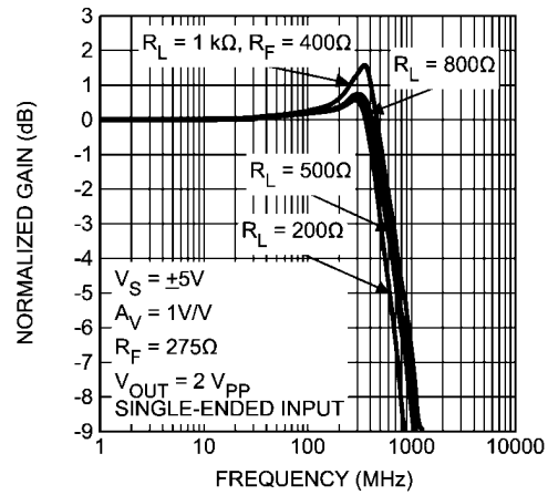
Frequency Response vs. Resistive Load
