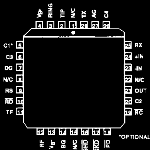
HC-5502B (PLCC) TOP VIEW
