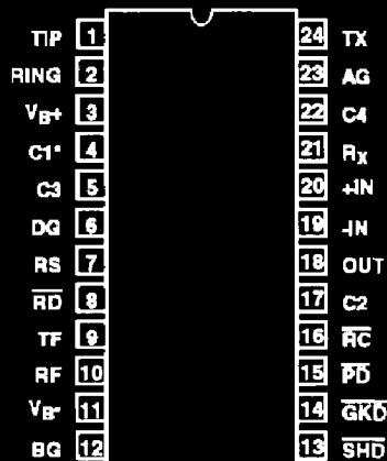
HC-5502B (PDIP, CDIP, SOIC) TOP VIEW
