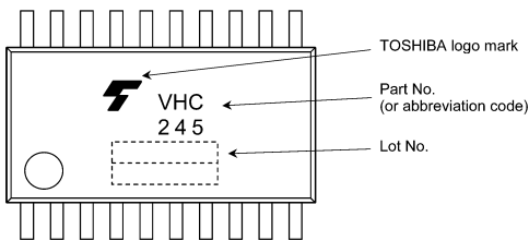
Fig. 6.2 Marking 2
