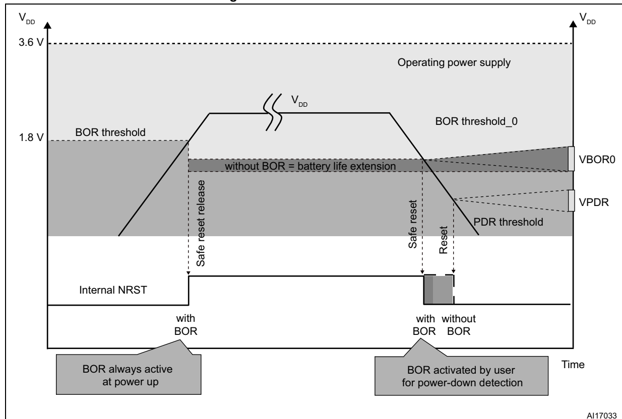
Figure 7. POR/BOR thresholds
