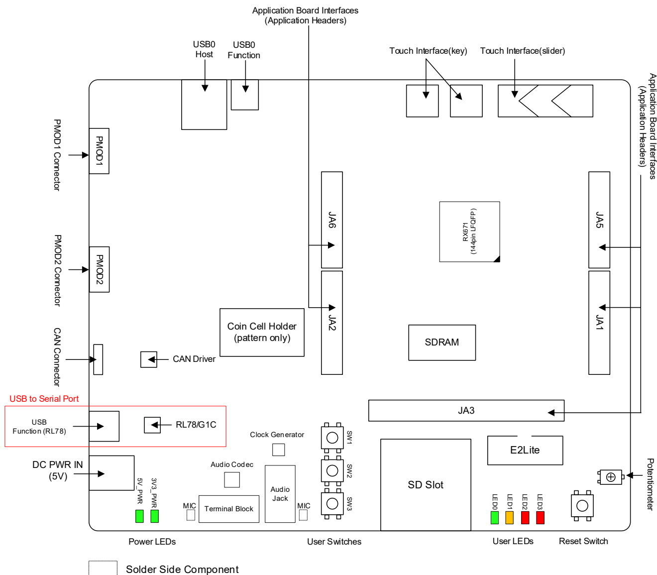
Figure 3-1: Board Layout
