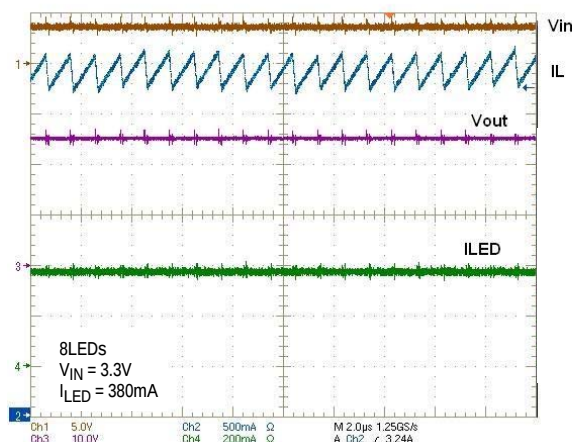
FIGURE 26. CURRENT LIMIT
