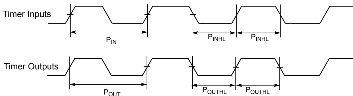
Figure 10-15 Timer Timing
