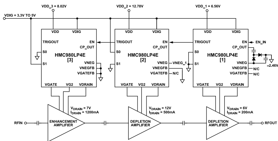
Figure 45. Daisy-Chain Operation
