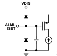
Figure 12. ALML, ISET Interface Schematic (Input)
