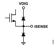
Figure 11. ISENSE Interface Schematic (Input)
