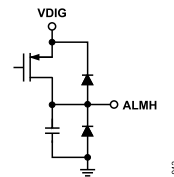
Figure 13. ALMH Interface Schematic (Input)
