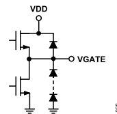
Figure 9. VGATE Interface Schematic (Output)
