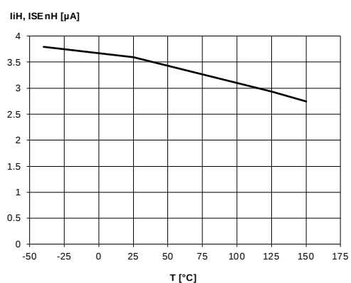
Figure 13: High level logic input current
