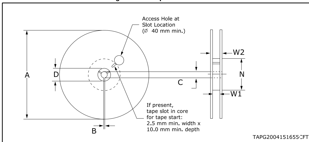
Figure 41: Octapak reel 13"
