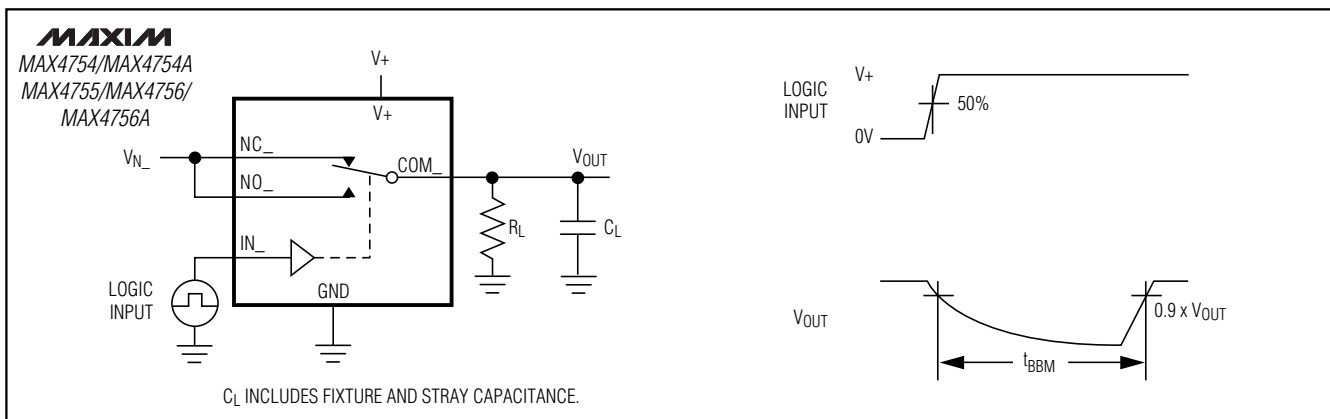
Figure 2. Break-Before-Make Interval
