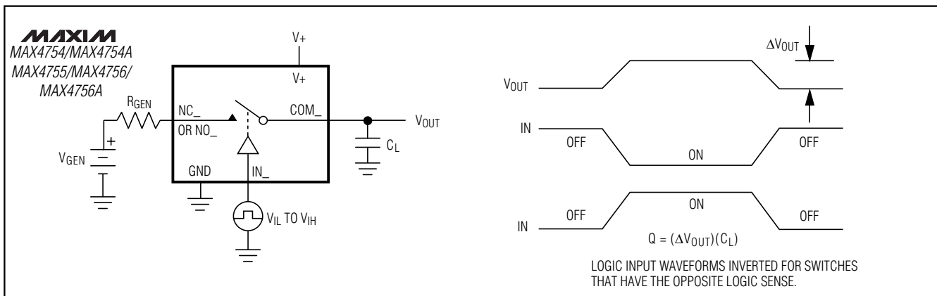
Figure 3. Charge Injection
