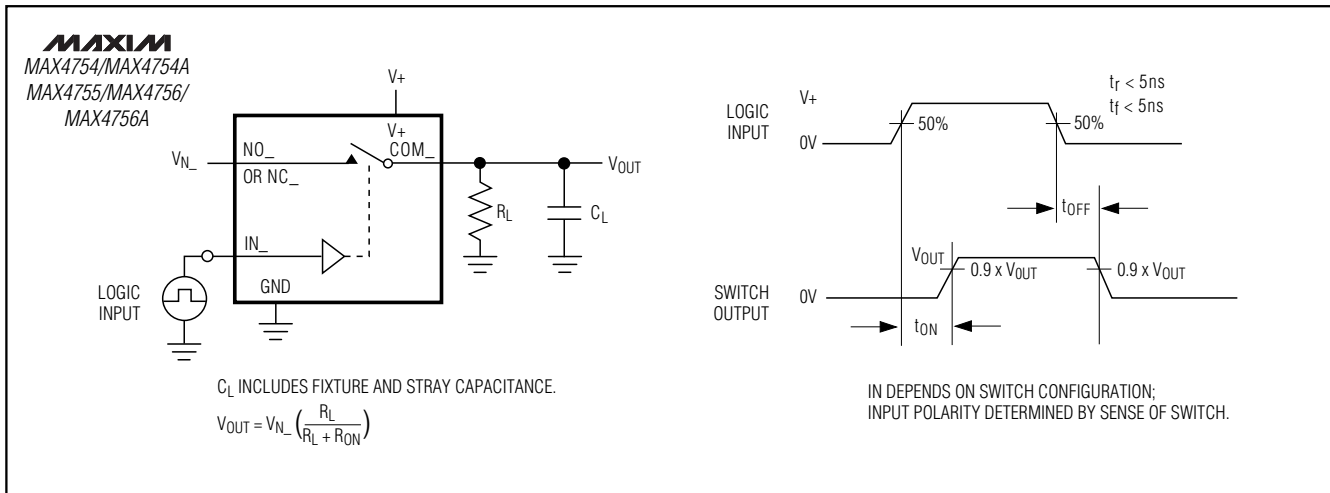
Figure 1. Switching Time
