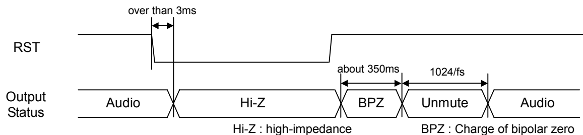
Figure 1. Reset Timing
