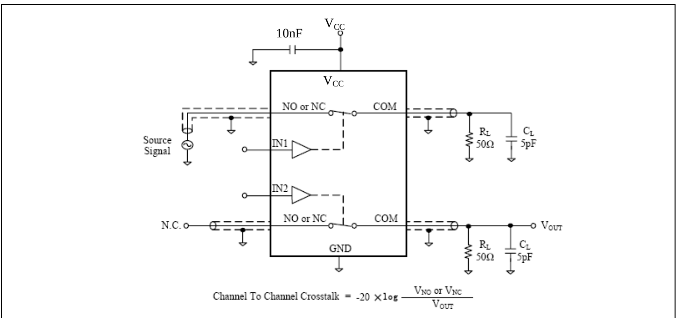
Figure 5. Channel-to-Channel Cross Talk
