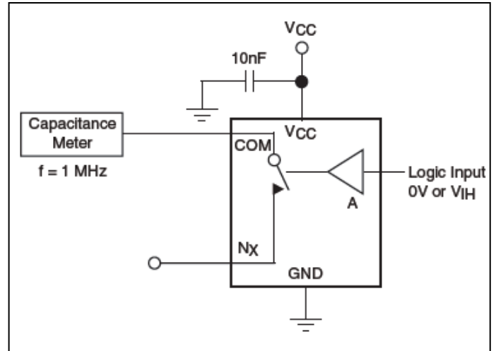
Figure 9. Channel On Capacitance
