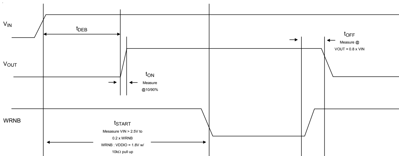
Figure 1. Timing for Power Up and Normal Operation
