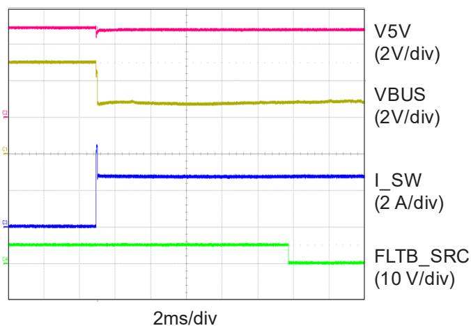
Source Mode Over Current Protection (Load = 1.2\Omega )
