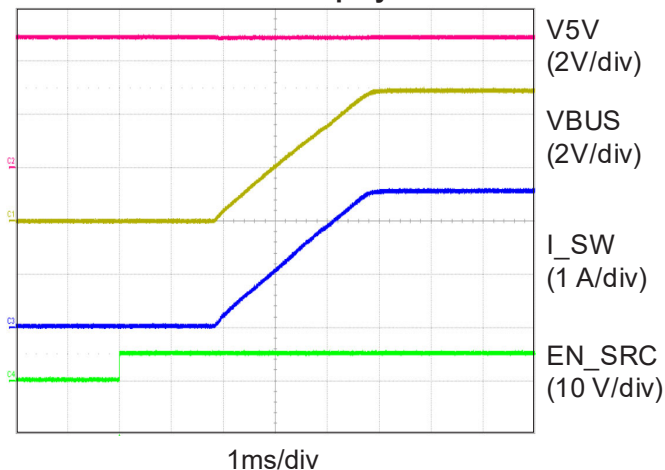
Source Mode Start Up by Enable
