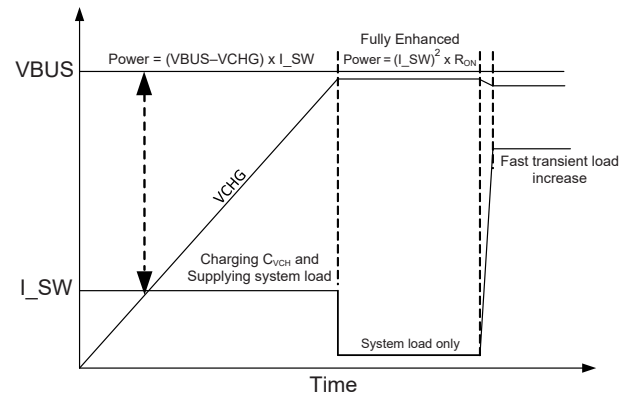
Figure 8. Soft-Start Power Dissipation
