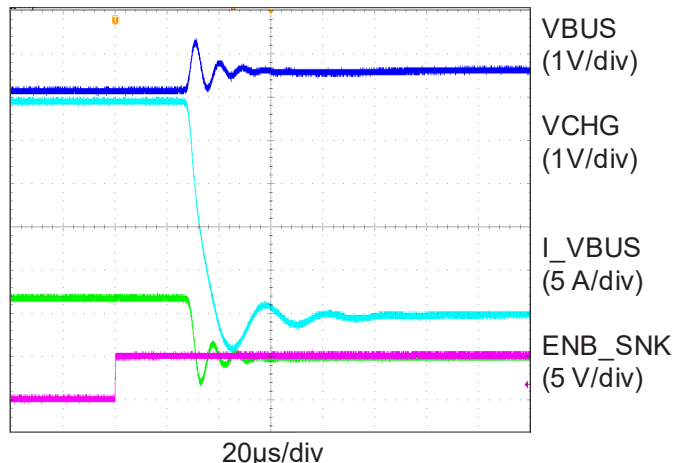
Shutdown ( V_{BUS}=20\text{V} , I_{LOAD}=8\text{A} )
