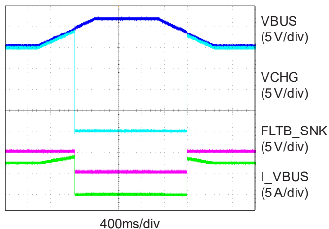
Sink Mode Over-Voltage Protection
