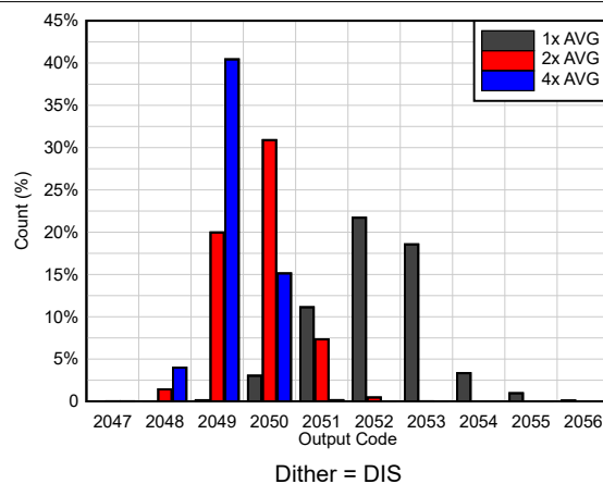
Figure 6-95. DC Offset Histogram
