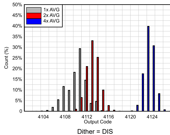
Figure 6-43. DC Offset Histogram
