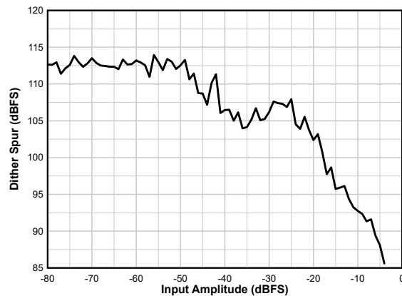
F_{IN} = 900 MHz, Figure 6-80. Dither Spur vs A_{IN}
