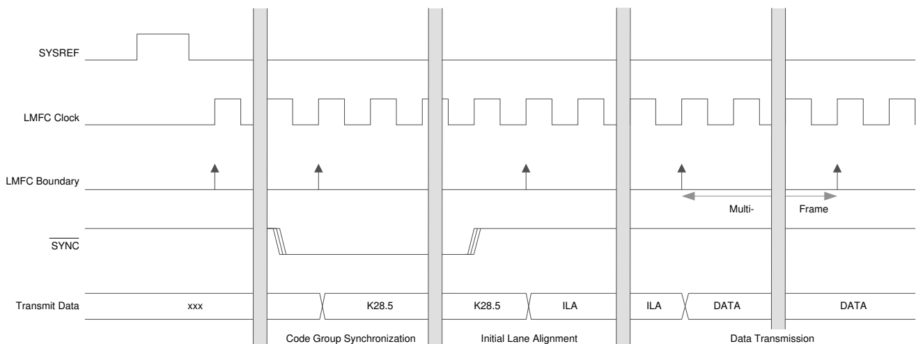
Figure 7-42. JESD204B Internal Timing Diagram
