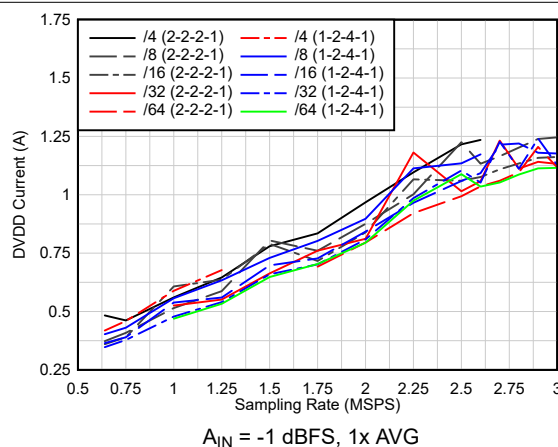
Figure 6-99. Current vs Sampling Rate vs Real Decimation
