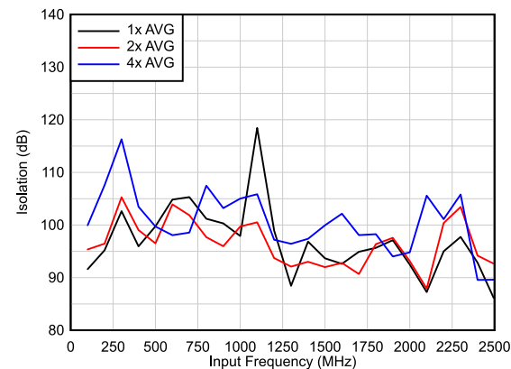
Figure 6-40. Isolation vs Input Frequency
