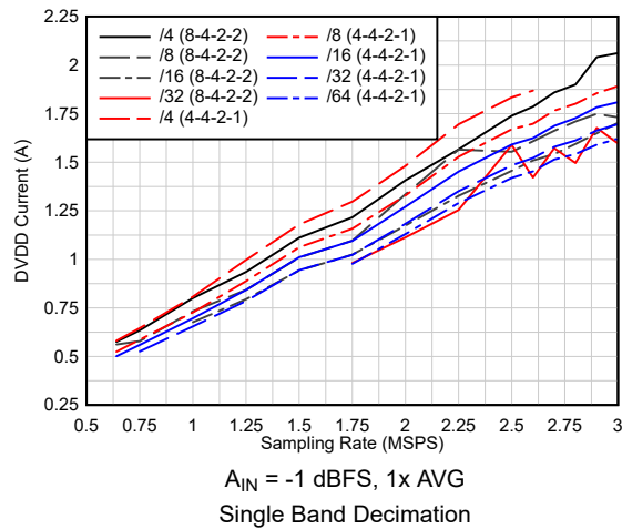
Figure 6-100. Current vs Sampling Rate vs Complex Decimation
