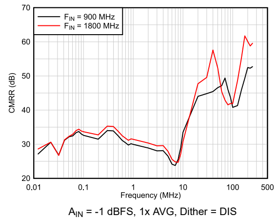
Figure 6-44. CMRR
