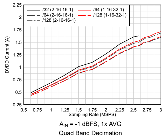
Figure 6-105. Current vs Sampling Rate vs Complex Decimation
