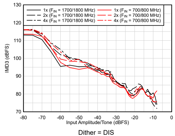
Figure 6-32. IMD3 Performance vs A_{IN}
