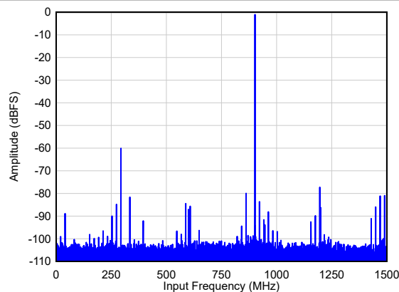
Figure 6-64. Single Tone FFT at F_{IN} = 900 MHz
