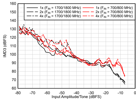
Figure 6-82. AC Performance vs A_{IN}
