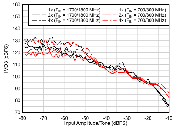
Figure 6-83. AC Performance vs A_{IN}
