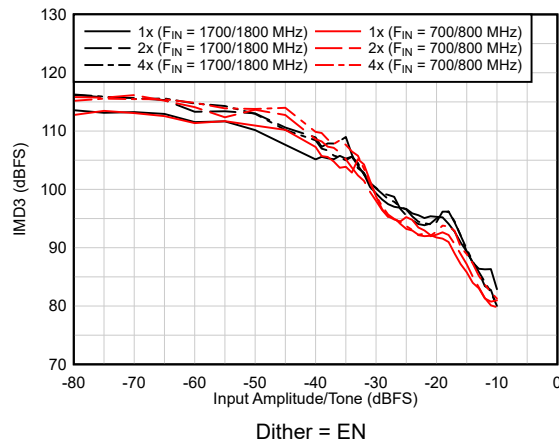
Figure 6-33. IMD3 Performance vs A_{IN}
