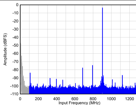
Figure 6-14. Single Tone FFT at F_{IN} = 900 MHz
