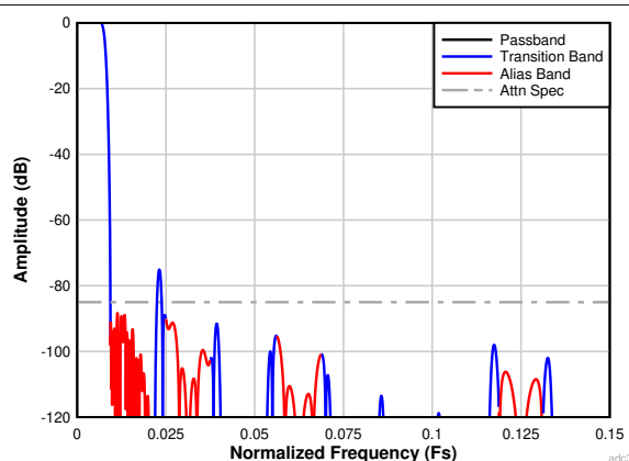
Figure 7-33. Complex Decimation by 64 Filter Response
