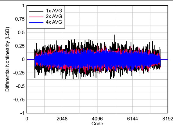
Figure 6-42. DNL vs Code
