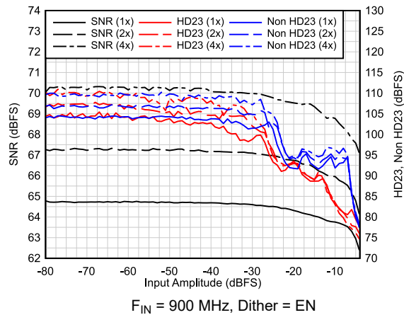
Figure 6-31. AC Performance vs A_{IN}
