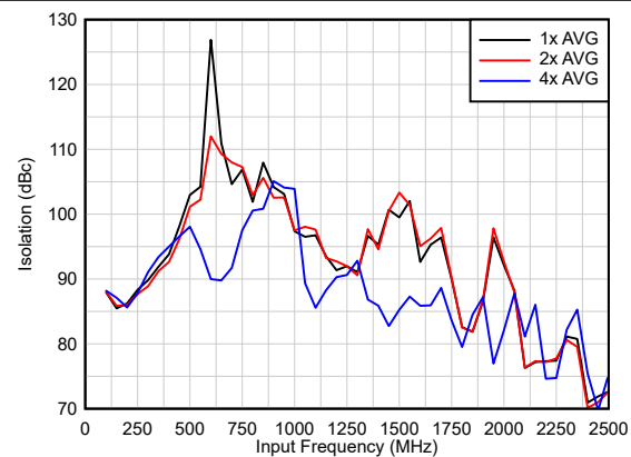
Figure 6-92. Isolation vs Input Frequency
