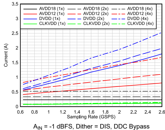
Figure 6-45. Current vs Sampling Rate vs Averaging
