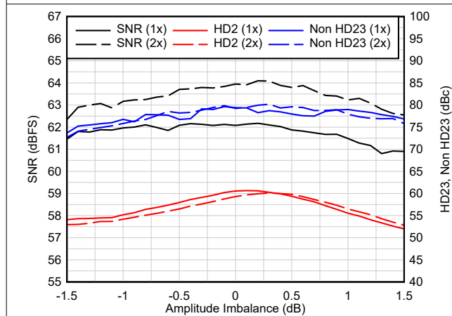
Figure 7-5. Amplitude Imbalance - 3.0 GSPS
