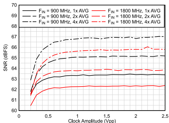
Figure 7-12. SNR vs Clock Amplitude (Dither OFF)
