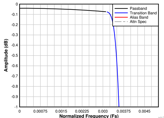
Figure 7-37. Decimation by 128 Passband Ripple Response
