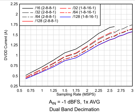
Figure 6-103. Current vs Sampling Rate vs Complex Decimation
