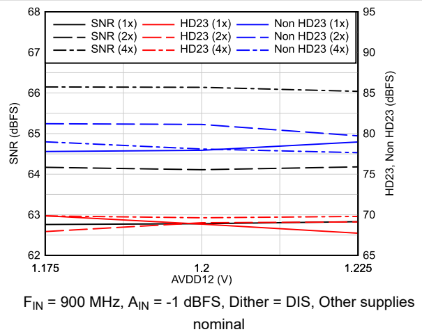
Figure 6-36. AC Performance vs AVDD12
