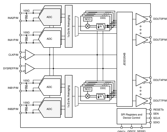
Block Diagram
