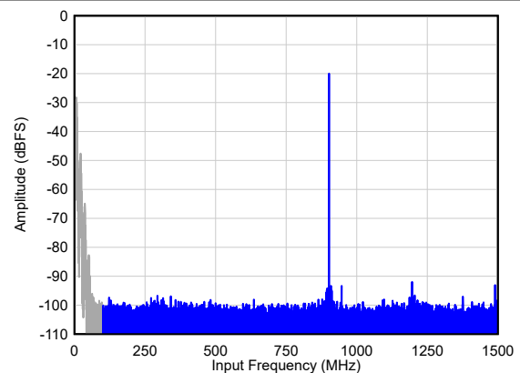
Figure 6-67. Single Tone FFT at F_{IN} = 900 MHz
