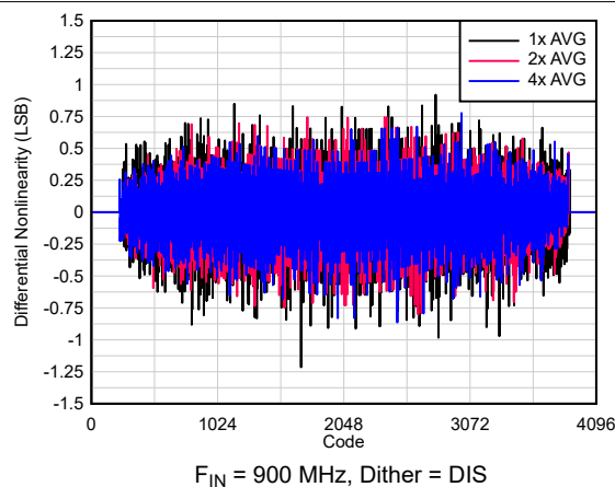
Figure 6-94. DNL vs Code
