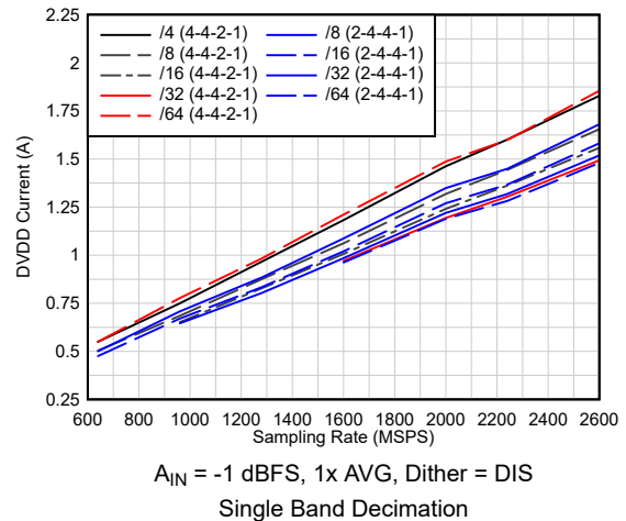
Figure 6-46. Current vs Sampling Rate vs Decimation
