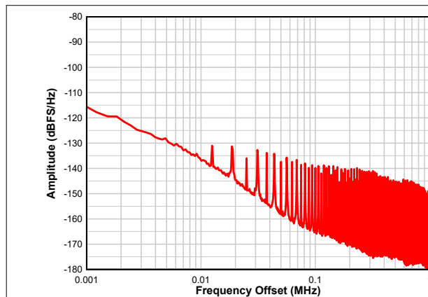
Figure 7-8. Dither Close-Up
