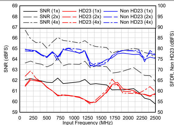
A_{IN} = -1 dBFS, Dither = DIS Figure 6-78. AC Performance vs F_{IN}
