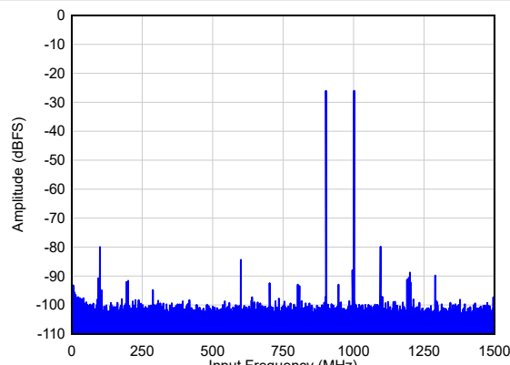
IMD3 = 54 dBc A_{IN} = -26 dBFS/tone, 1x AVG, Dither = DIS Figure 6-76. Two Tone FFT at F_{IN} = 900/1000 MHz
