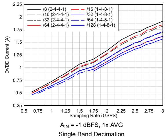
Figure 6-101. Current vs Sampling Rate vs Complex Decimation
