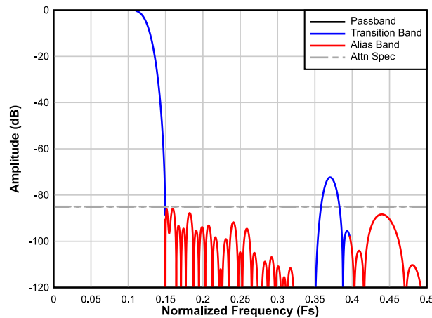
Figure 7-24. Complex Decimation by 4 Filter Response
