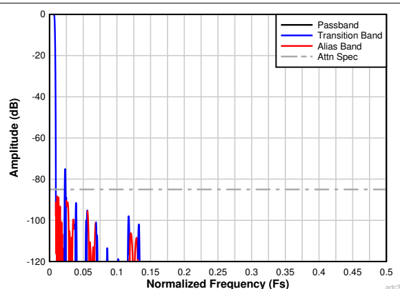
Figure 7-32. Complex Decimation by 64 Filter Response
