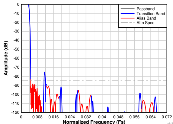
Figure 7-36. Complex Decimation by 128 Filter Response
