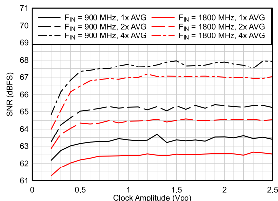
Figure 7-13. SNR vs Clock Amplitude (Dither ON)
