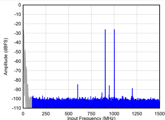
IMD3 = 71 dBc A_{IN} = -26 dBFS/tone, 1x AVG, Dither = EN Figure 6-77. Two Tone FFT at F_{IN} = 900/1000 MHz
