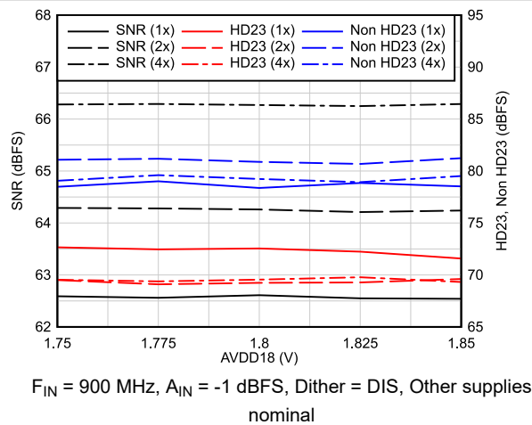
Figure 6-35. AC Performance vs AVDD18
