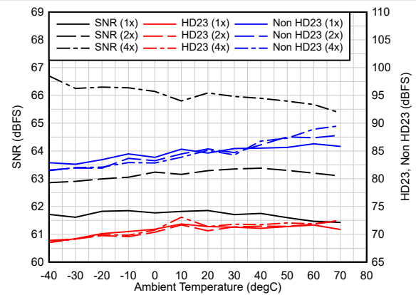
Figure 6-89. AC Performance vs Temperature
