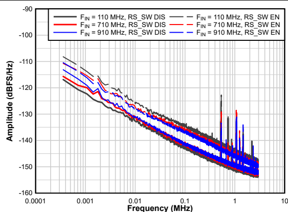
Figure 7-10. Amplitude Noise vs Input Frequency
