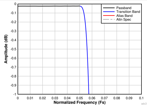
Figure 7-27. Decimation by 8 Passband Ripple Response
