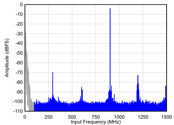
Figure 6-65. Single Tone FFT at F_{IN} = 900 MHz
