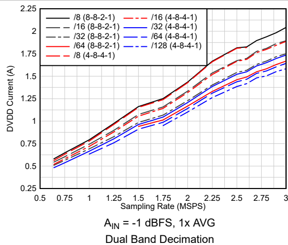
Figure 6-102. Current vs Sampling Rate vs Complex Decimation
