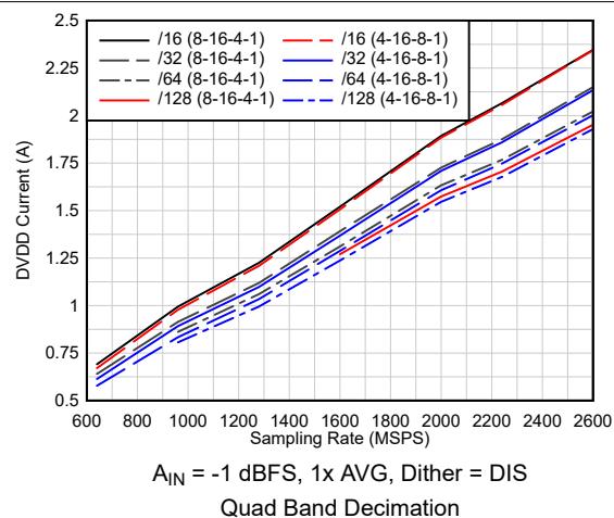
Figure 6-50. Current vs Sampling Rate vs Decimation
