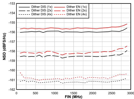
A_{IN} = -20 dBFS Figure 6-81. NSD Performance vs F_{IN}
