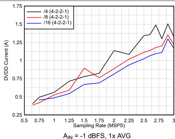
Figure 6-98. Current vs Sampling Rate vs Real Decimation
