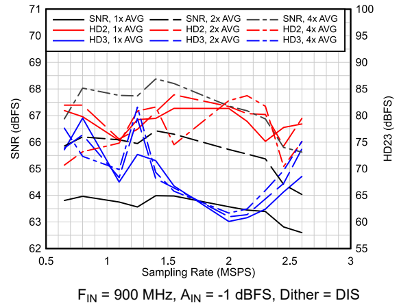
Figure 6-34. AC Performance vs F_S
