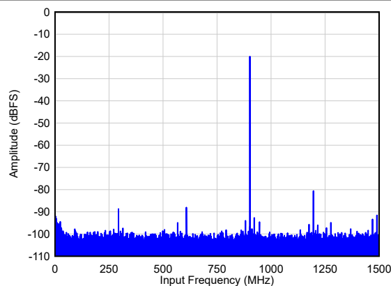
Figure 6-66. Single Tone FFT at F_{IN} = 900 MHz
