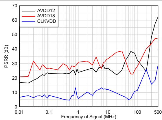
Figure 8-5. Power Supply Rejection Ratio (PSRR) vs Frequency
