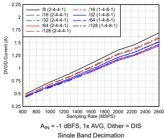
Figure 6-47. Current vs Sampling Rate vs Decimation
