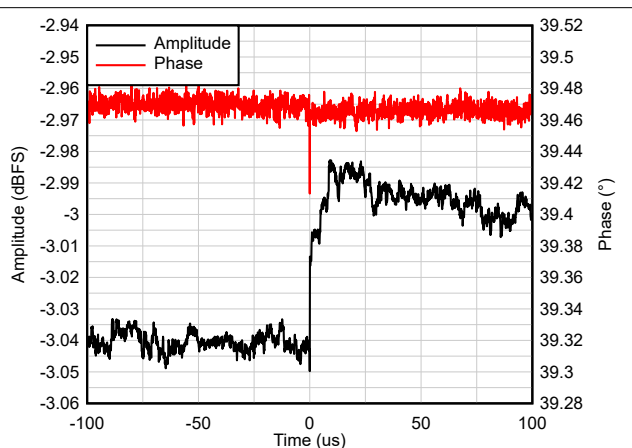
Figure 7-22. Amplitude and Phase vs Time
