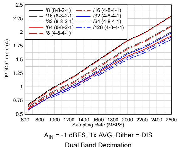
Figure 6-48. Current vs Sampling Rate vs Decimation
