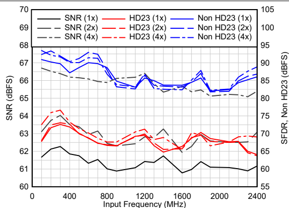
A_{IN} = -4 dBFS, Dither = EN Figure 6-79. AC Performance vs F_{IN}
