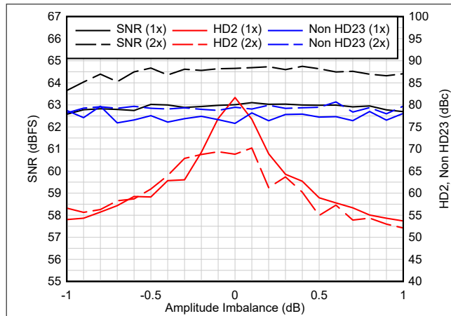
Figure 7-3. Amplitude Imbalance - 2.6 GSPS
