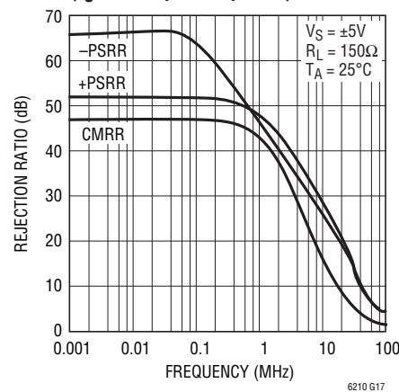
CMRR and PSRR vs Frequency ( I_S = 3mA per Amplifier)
