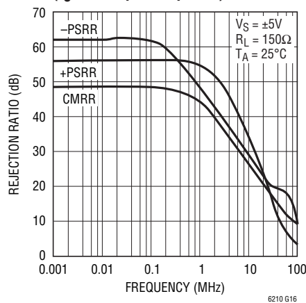
CMRR and PSRR vs Frequency ( I_S = 6mA per Amplifier)
