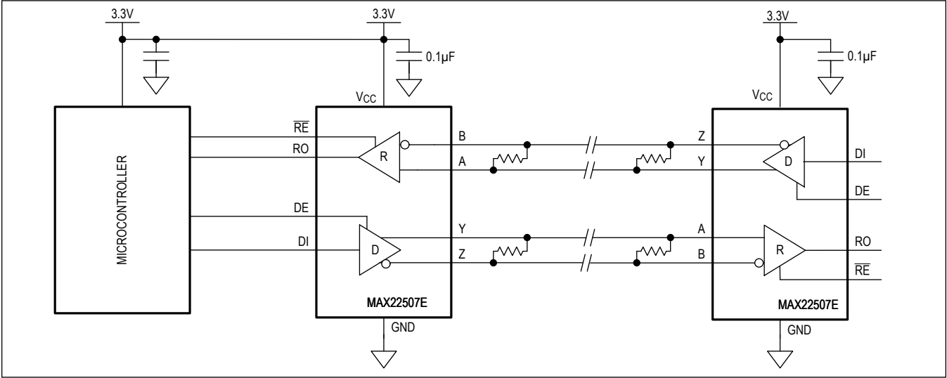
Full Duplex Point-to-Point Network
