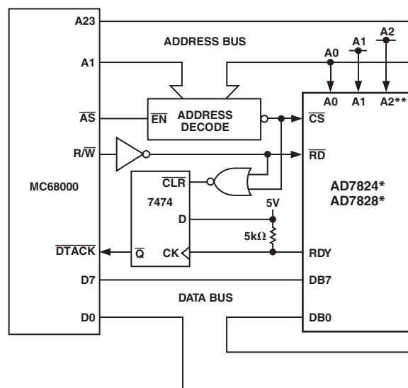
Figure 17. AD7824/AD7828–MC68000 Interface
