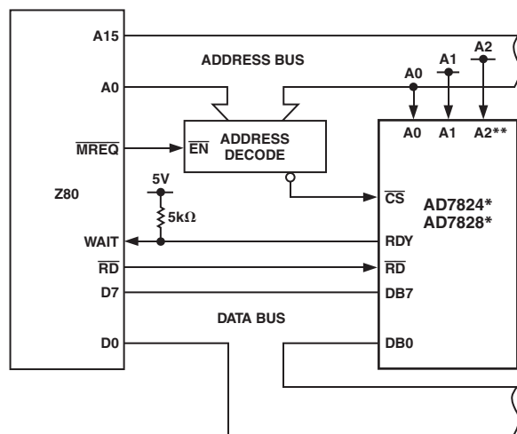
Figure 16. AD7824/AD7828–Z80 Interface
