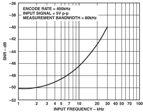
TPC 3. Signal-to-Noise Ratio vs. Input Frequency
