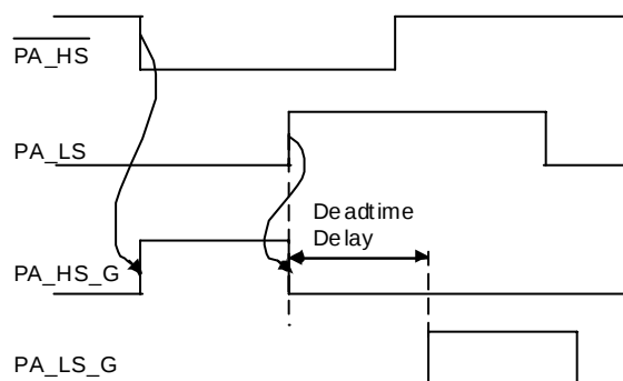
Figure 11. Edge Sensitive Logic Inputs (Phase A)
