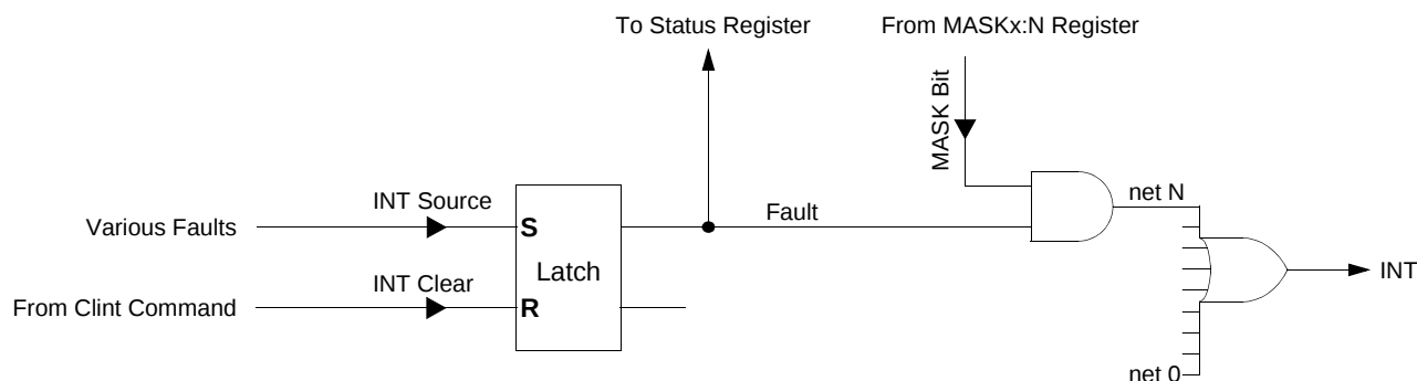
Figure 15. Interrupt Handling
