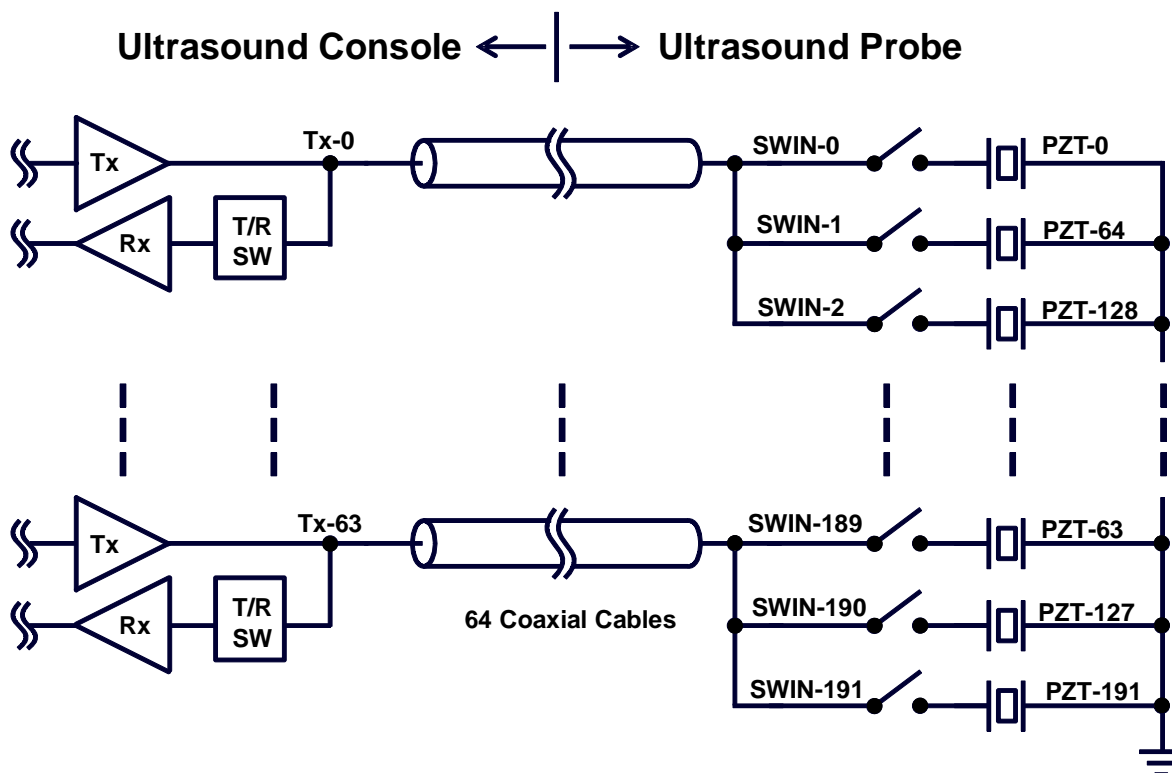
Figure 16: The MP4835A Inside the Ultrasound Probe Head
