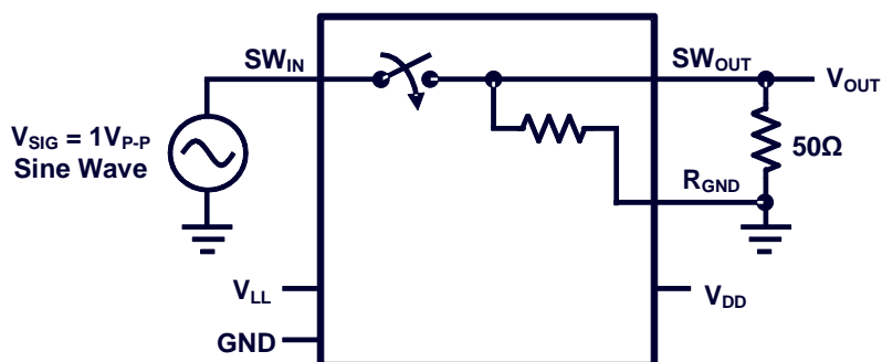
Figure 8: Test Circuit 8
