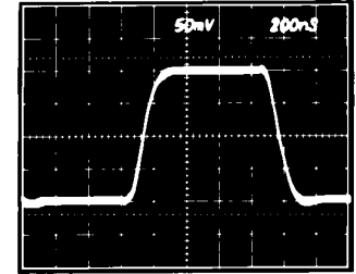
Figure 24c. Unity Gain Inverter Pulse Response (Small Signal)
