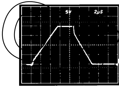
Figure 21a. Unity Gain Follower Pulse Response (Large Signal)
