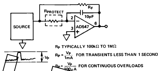
Figure 30. Input Protection
