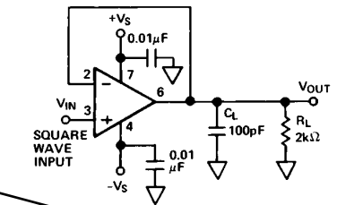
Figure 21d. Unity Gain Follower-AD542/AD547
