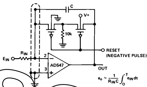
Figure 35. Low Drift Integrator and Low Leakage Guarded Reset
