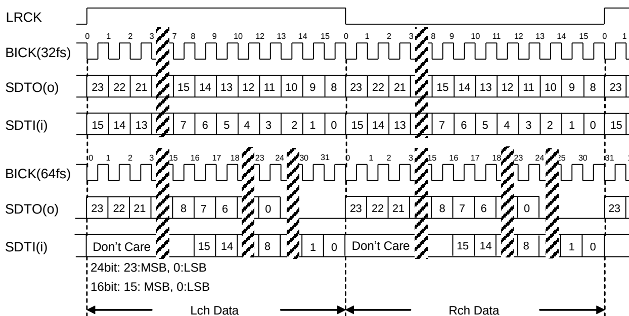
Figure 22. Mode 1 Timing
