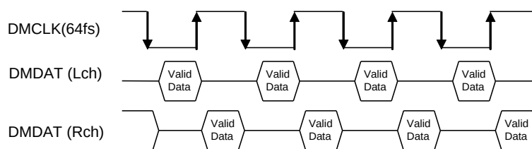
Figure 29. Data In/Output Timing with Digital MIC (DCLKP bit = “0”)
