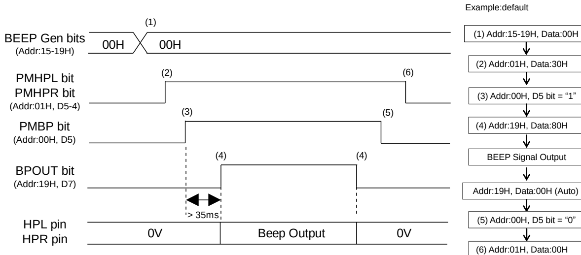
Figure 59. "BEEP Generator → Headphone-Amp" Output Sequence
