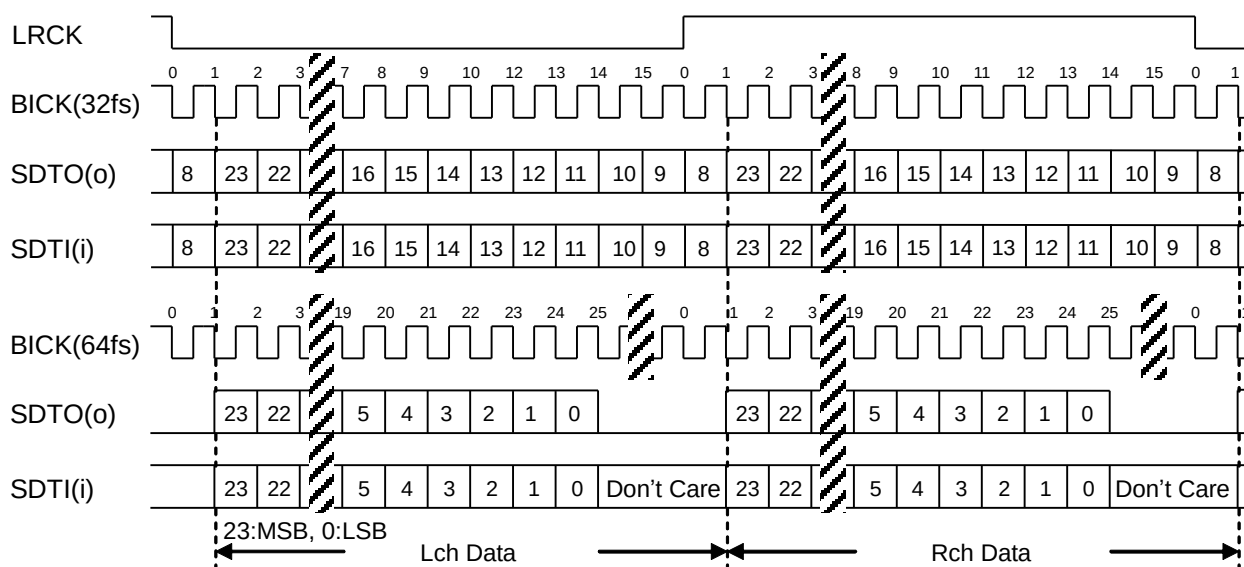
Figure 24. Mode 3 Timing
