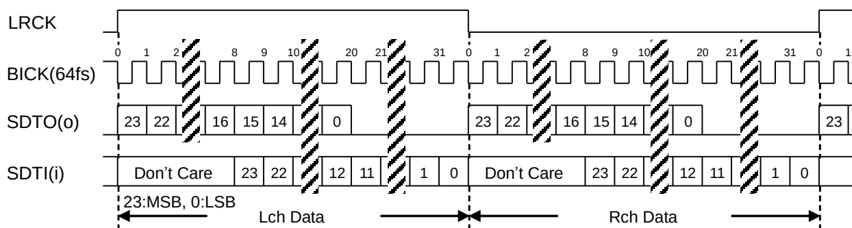
Figure 21. Mode 0 Timing
