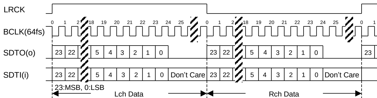
Figure 23. Mode 2 Timing
