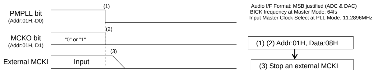
Figure 63. Clock Stopping Sequence (1)
