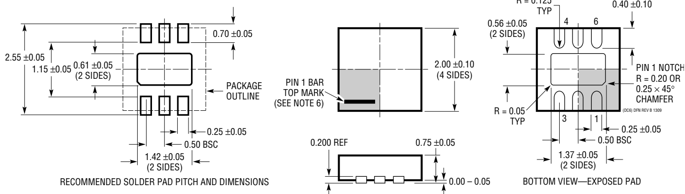
DC6 Package 6-Lead Plastic DFN (2mm × 2mm) (Reference LTC DWG # 05-08-1703 Rev B)
