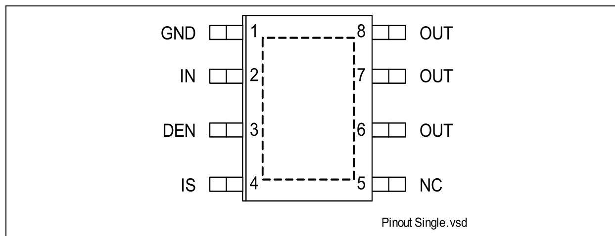
Figure 2 Pin Configuration
