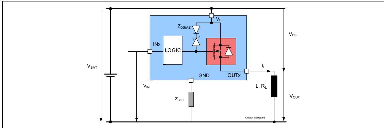
Figure 10 Output Clamp
