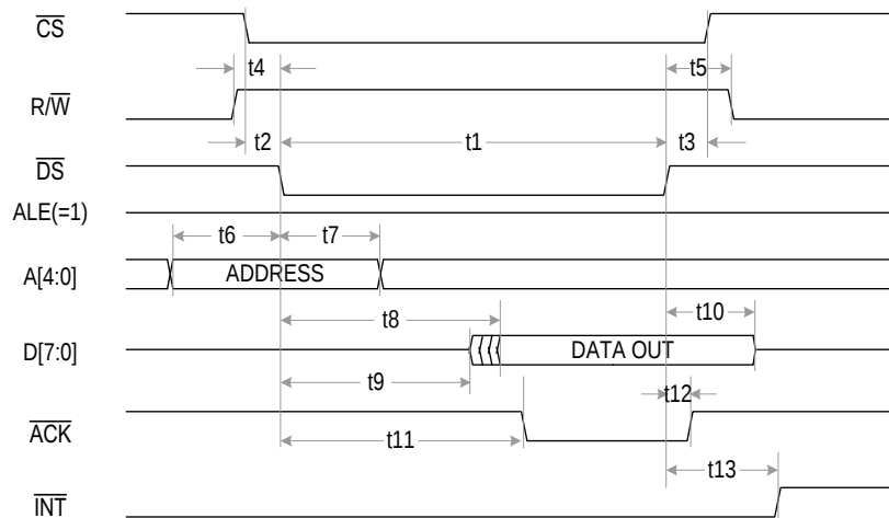
Figure-34 Non-Multiplexed Motorola Mode Read Timing
